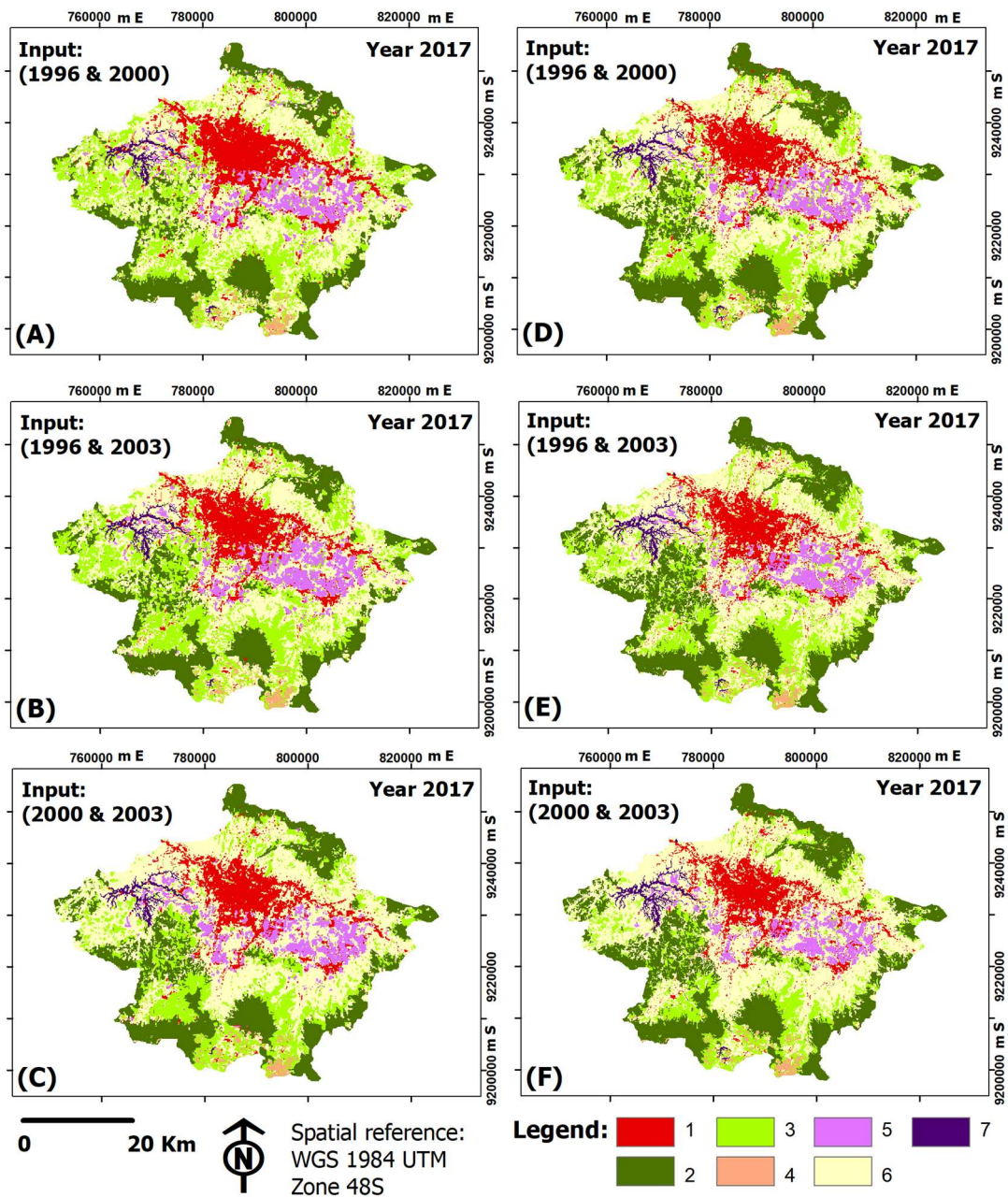
Figure 8. The results of simulating and predicting LULC in 2017 based on the combination input data pairs for 1996, 2000 and 2003: A), B) and C) LULC in 2017 from the Markov-CA model without integration of the landform-based model; D), E) and F) LULC in 2017 from the integration of the Markov-CA and landform-based models. Class 1: built land; class 2: primary forest; class 3: secondary forest and mixed garden; class 4: plantation; class 5: wet agricultural land; class 6: dryland farming; class 7: water body
