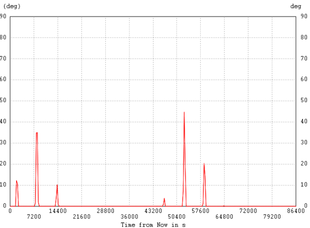
Fig. 9. Communication duration between the satellite and the ground station (simulation).
