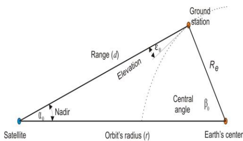
Fig. 4. Ground station geometry.
