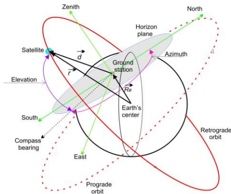
Fig. 3. Horizon plane and orbits.
