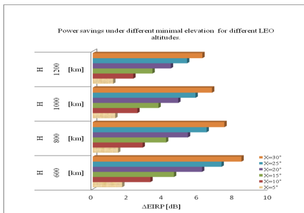
Fig. 10. Power savings ( \Delta EIRP ).
