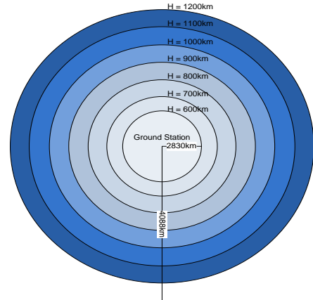
Fig. 5. Ideal horizon plane for different altitudes.
