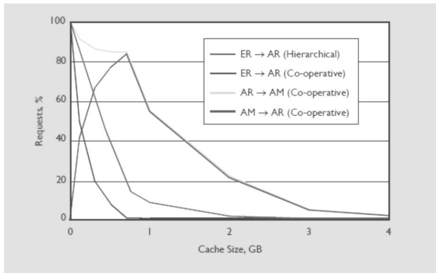
Fig. 7. Relative load on the links between ER, AR and AM
