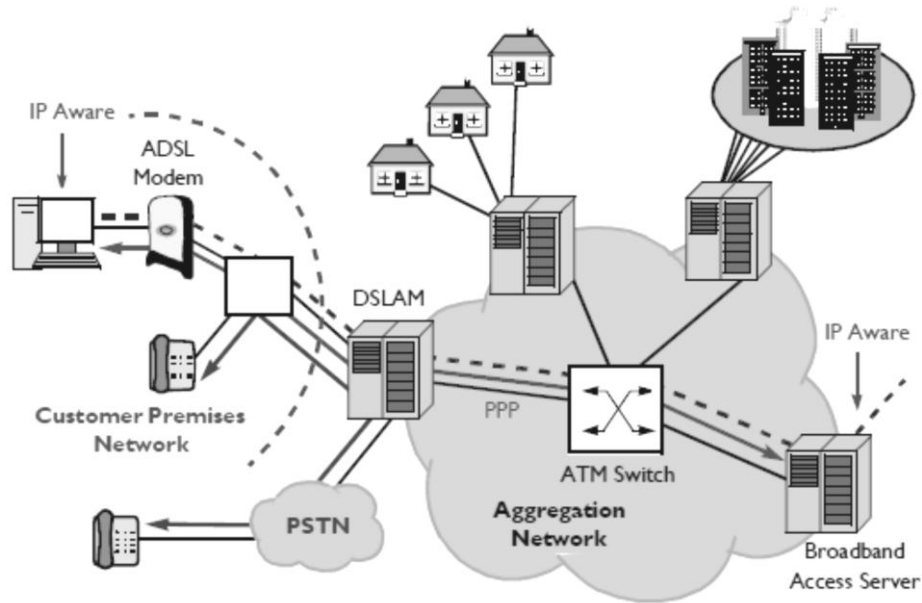
Fig. 2. Current access networks
