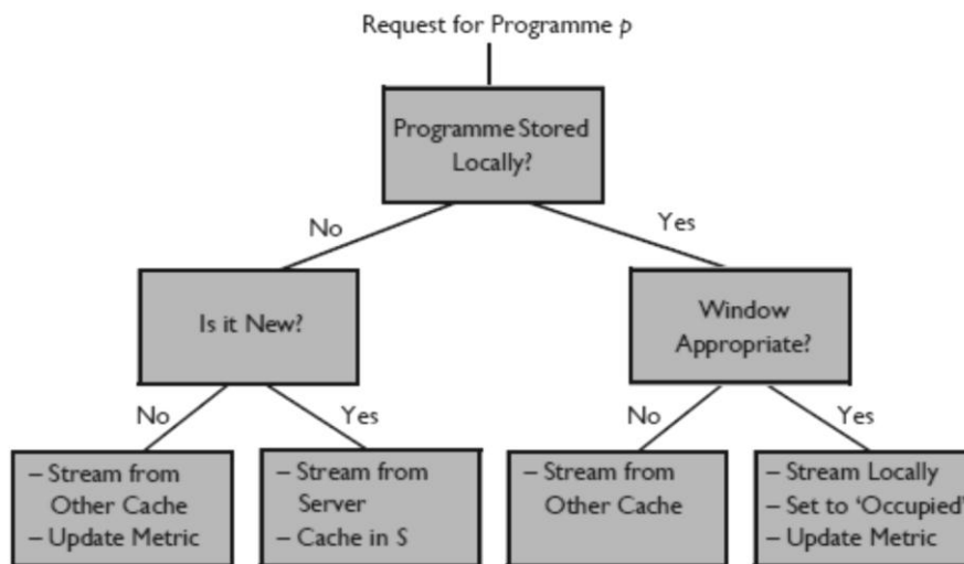
Fig. 6. Basic principle of the tsTV caching algorithm at each proxy
