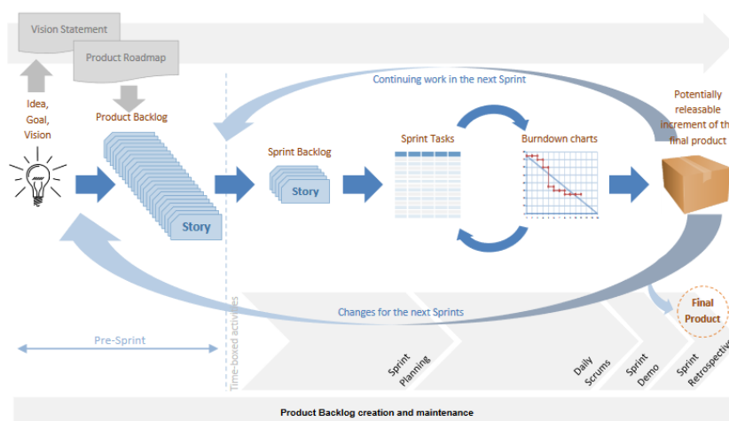
Gambar 2. Scrum Timeline
