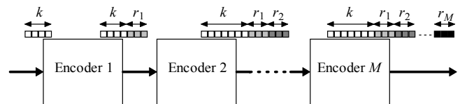
Fig. 1. Serial concatenation in M-SC-MPC codes.
