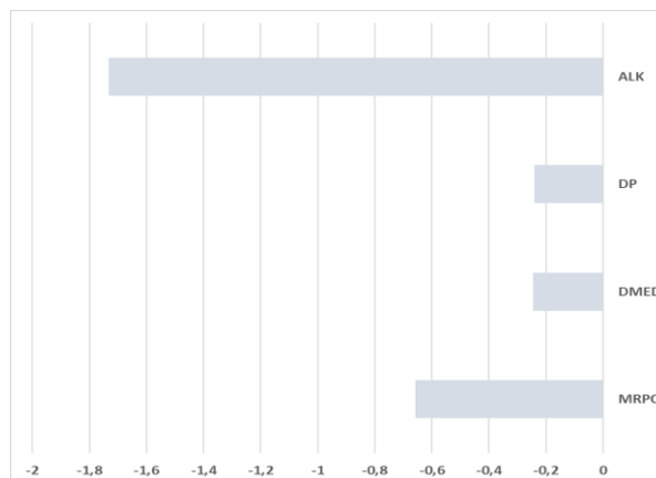
Fig. 8 Arc elasticity chart illustrating the effect of selected independent variables on the relative road fatality rate RFR in model 5.2.
