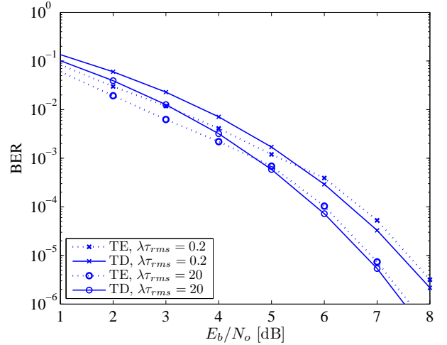
Figure 7. BER comparison of turbo detector and turbo equalizer of [7] for different values of \lambda\tau_{rms} . The normalized data rate is R_b\tau_{rms} = 0.1 .
