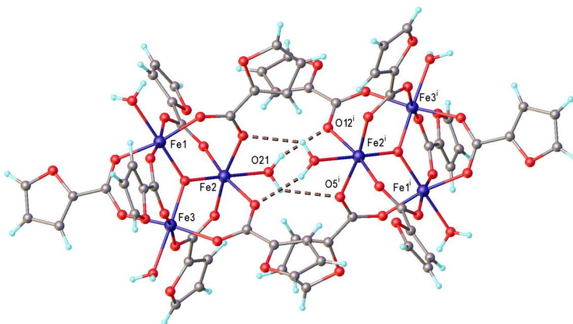
Figure 2. Two H-bonded complexes as a self-assembled centrosymmetric unit. Symmetry transformation used to generate equivalent atoms: -x, 2-y, 1-z .
