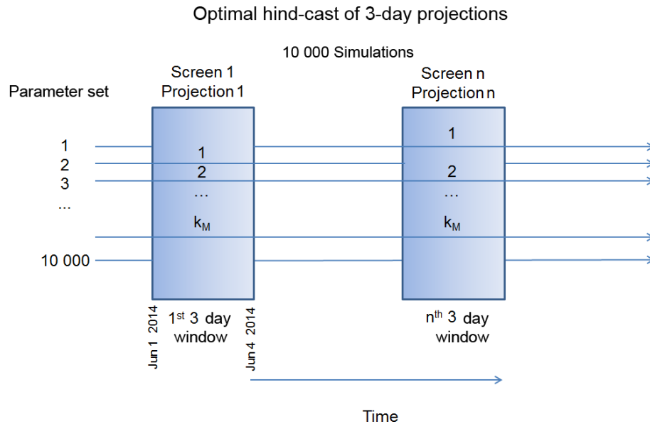
Figure 4. Schematic of P-SET for the optimal hindcast of 3-day projections used in this study; 10 000 simulations are run continuously through the MESH model, of which the screen chooses a number ( k_M ) for the hindcast analysis. The process is then repeated for subsequent screening periods.
