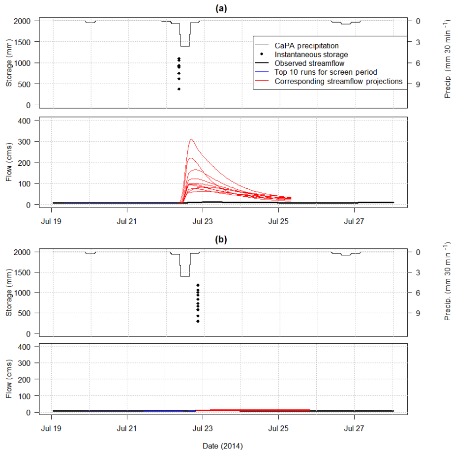
Figure 8. A single screen-projection period for two neighbouring time periods. For the two sub-plots in (a) the projection begins at 07:00 LT (local time), 22 July 2014 (12:00 UTC). For the two sub-plots in (b) the projection begins at 19:00 LT, 22 July 2014 (00:00 UTC, 23 July). The upper plot of each sub-figure shows CaPA precipitation and instantaneous storage. The lower plot shows observed streamflow (black), the top 10 runs for the screening period (blue), and the corresponding streamflow projections (red).
