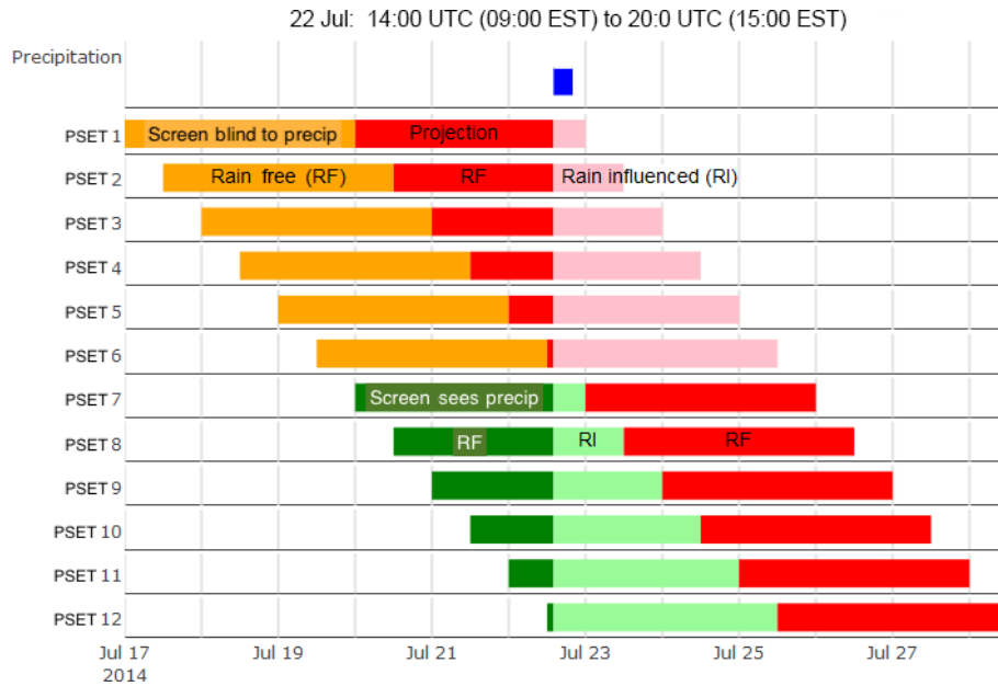
Figure 3. Preceding streamflow screen and projection periods for 17 to 28 July 2014 using hourly streamflow. This figure is fully explained in Sect. 2.7.2 and 2.8.2.
