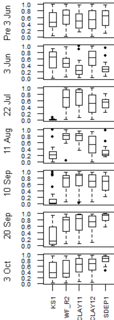
Figure 9. Importance of (normalized) parameters that see precipitation. The top set of box-plots shows that none of the top parameter sets have identifiable parameter values prior to the 3 June 2014 precipitation event. This result is similar to all parameter sets immediately prior to precipitation events that do not see the events. The remaining sets of box-plots show the parameter ranges for the top simulations during precipitation events.
