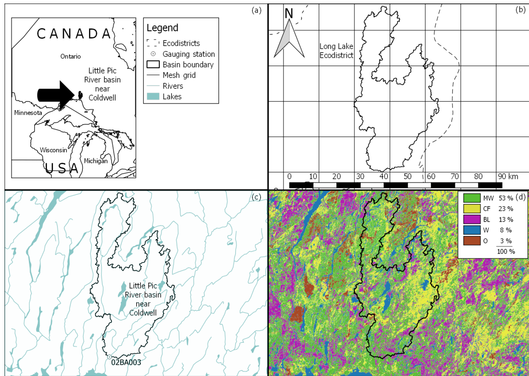
Figure 2. Little Pic River basin near Coldwell, Ontario, Canada. (a) Location of the basin and legend, (b) basin outline with respect to ecodistrict, (c) river network and gauge location (02BA003), and (d) land cover (MW is mixed wood, CF is coniferous forest, BL is broadleaf forest, W is water, and O is other).
