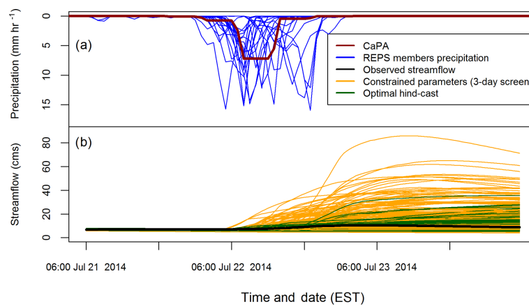
Figure 11. Results of the H-EPS for the 3-day period beginning at 06:00 EST (Eastern Standard Time) on 21 July 2014. The reddish brown line in (a) is the Canadian Precipitation Analysis (CaPA), while the blue lines represent the 20 Regional Ensemble Prediction System (REPS) precipitation traces. The single black line in (b) is the observed streamflow. The orange and green lines show the 200 H-EPS streamflow traces for the projection periods of the constrained parameter with a preceding 3-day streamflow screen, and the optimized hind-cast.
