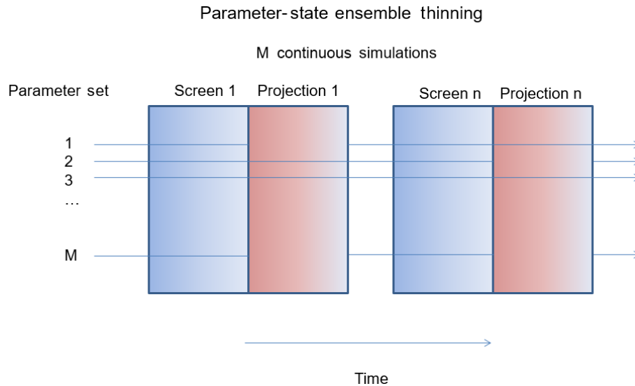
Figure 1. Schematic of the P-SET approach. M simulations are run continuously from a model, of which the screen chooses a number from which to analyse a projection. The process is then repeated for subsequent screening periods, noting that the M simulations run continuously through the previous projection periods even though they are not all selected for the previous projection period analysis.
