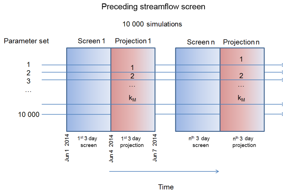
Figure 5. Schematic of P-SET for the preceding streamflow screen; 10 000 simulations are run continuously through the MESH model, of which the screen chooses a number ( k_M ) from which to analyse a projection. The process is then repeated for subsequent screening periods, noting that the M simulations run continuously through the previous projection periods even though they are not all selected for the previous projection period analysis.
