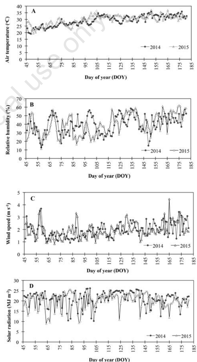
Figure 1. Daily average air temperature (A), relative humidity (B), wind speed at 2 m height (C), and incoming solar radiation (D) measured at the experimental site for the 2014 and 2015 dry seasons.
