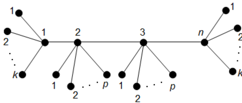
Figure 3. The thorn path P_{n,p,k} .
