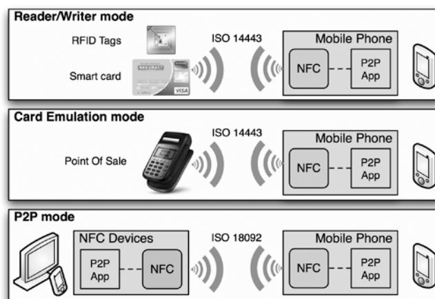
Fig. 1. NFC operating modes and standards
