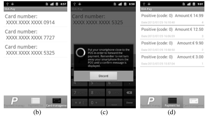
Fig. 6. Some screenshots of the IDA-Pay prototype: (a) the cashier inserts the amount into the IDA-Pay POS application, (b) the buyer starts the IDA-Pay App and taps a credit card from the configured credit card list, (c) the app asks the buyer to touch the smartphone to the POS NFC reader, (d) the payment response is stored into the payments' archive.
