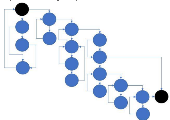
Gambar 7. Control Flow Graph Usulan Algoritma
