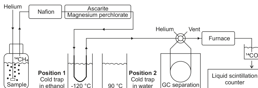
Figure 2. Schematic view of the methane stripping-oxidation line. Position 1 (displayed): the cold trap is placed in a -120^{\circ}\text{C} ethanol bath to retain the hydrocarbons. Position 2: the cold trap is transferred into a water bath at 90^{\circ}\text{C} to release the hydrocarbons towards the gas chromatograph (GC). A detailed description is included in Sect. S2.
