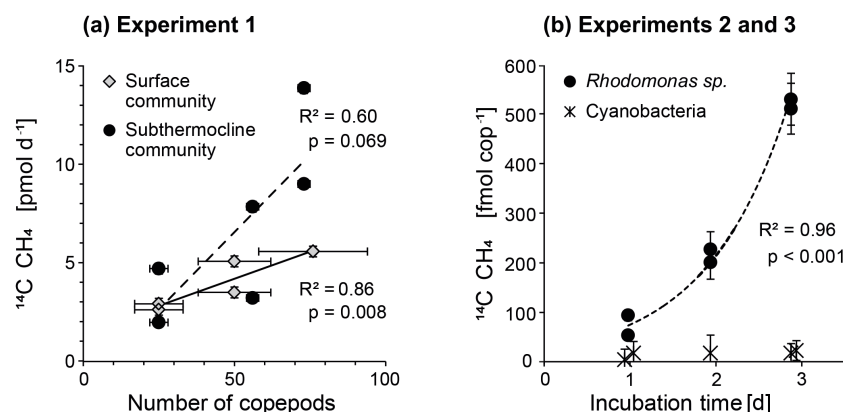
Figure 6. (a) Experiment 1: methane production as a function of the number of copepods in the surface (dominated by Acartia spp.) and subthermocline zooplankton communities (dominated by Temora longicornis ). (b) Experiments 2 and 3: copepod-specific methane production over time when using the cryptophyte alga Rhodomonas sp. (experiment 2) or the cyanobacterium Nodularia spumigena (experiment 3) as food sources.
