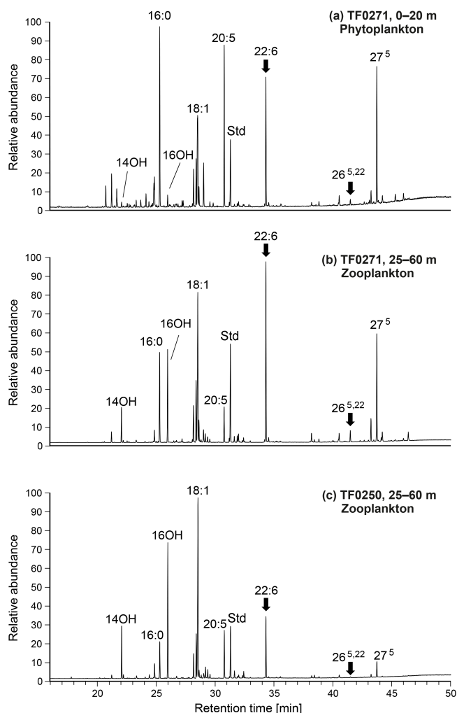
Figure 11. GC–MS chromatograms of neutral lipids (methyl ester/TMS derivatives) from mixed-layer phytoplankton (a) and subthermocline zooplankton (b) at station TF0271 (with a distinct subthermocline methane enrichment). Data from subthermocline zooplankton at TF0250 (without a distinct subthermocline methane enrichment) are shown as a reference (c). Main compounds are labelled and interpreted as follows (see text for further discussion); 16:0, n -hexadecanoic acid (unspecific, high in bacteria); 14OH / 16OH, n -tetradecanol and n -hexadecanol (copepod wax esters); 18:1, oleic acid (unspecific, high in heterotrophs but also in (cyano)bacteria); 20:5, n -eicosapentaenoic acid (phytoplankton, high in diatoms); Std, internal standard; 22:6, n -docosahexaenoic acid (phytoplankton, high in Dinophyceae); 26 5,22 , 24-norcholesta-5,22-dien-3 \beta -ol (specific for Dinophyceae); 27 5 , cholesterol (unspecific, high in zooplankton, but also found in some algae including Dinophyceae). Compounds indicating contributions from Dinophyceae-derived lipids are highlighted with an arrow. Note enhanced levels of these biomarkers in T. longicornis -dominated zooplankton at the station with a distinct subthermocline methane enrichment (TF0271).
