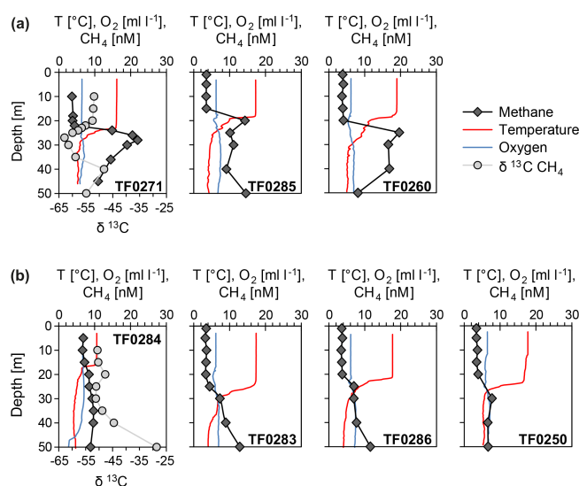
Figure 3. Vertical profiles of temperature ( T ), oxygen ( \text{O}_2 ) and methane ( \text{CH}_4 ) concentrations in the central Baltic Sea: (a) stations with a distinct, and (b) stations without a distinct subthermocline methane enrichment; stable carbon isotope values of methane ( \delta^{13}\text{C} ) are presented for station TF0284 (western Gotland Basin) and TF0271 (eastern Gotland Basin).
