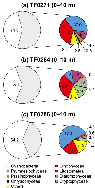
Figure 8. Surface phytoplankton community composition integrated over the upper 10 m of the water column ( \text{mg C m}^{-3} ) at stations with a distinct (a) and without a distinct (b, c) subthermocline methane enrichment. The grey shaded non-cyanobacteria community is described in detail in the coloured circles.
