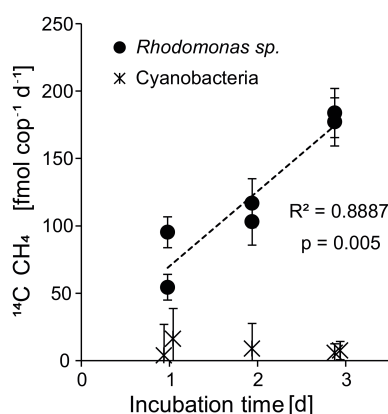
Figure 7. Experiments 2 and 3: copepod-specific methane production rates over time for the two food sources Rhodomonas sp. and cyanobacterium Nodularia spumigena .
