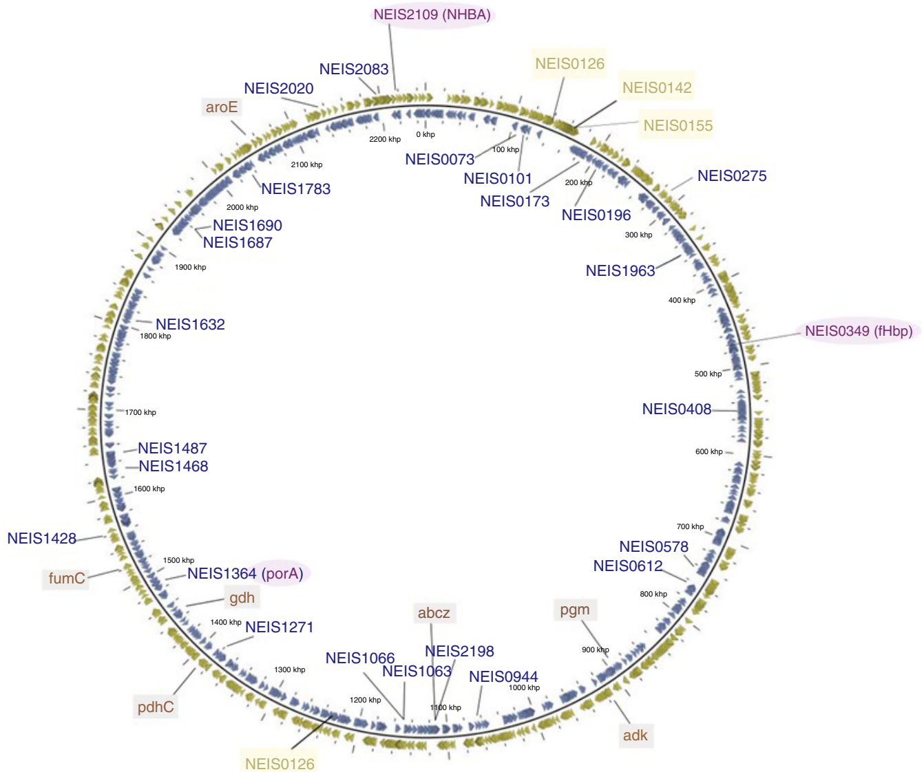
Figure 1. Representation of Neisseria meningitidis reference genome NZ05/33, drawn with Gview 29 . NZ05/33 is an ST41/44 outbreak strain from New Zealand. The MeNZB™ vaccine was developed from NZ98/254, another ST41/44 isolate from the same New Zealand outbreak. Chromosomal location of the genes encoding the proteins included in the Outer Membrane Vesicle peptide Typing (OMVT) scheme are shown in blue. Genes encoding four cytoplasmic proteins are shown in yellow boxes. The multilocus sequence typing loci are shown in brown boxes. The genes encoding the constituents of the Bexsero® Antigen Sequence Typing scheme are shown in purple ellipses, note that nadA is absent in this strain.
