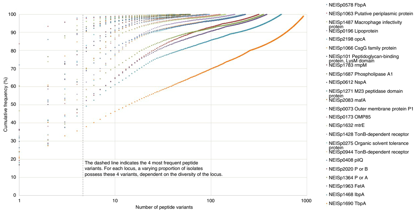
Figure 4. Distribution of Outer Membrane Vesicle peptide Typing (OMVT) variants in UK meningococcal disease isolates. The cumulative frequency distribution is shown for each locus in the OMVT scheme. For each peptide, it shows the proportion of the 3506 isolates that were annotated with each successive peptide variant. The grey dashed line indicates the proportion of isolates within the dataset which possess the four most frequent variants. The distribution is highly skewed, as for FbpA (NEISp0578), Putative periplasmic protein (NEISp1063), Mip/FkpA (NEISp1487) and PldA (NEISp1687) four variants annotated >90% of isolates, contrasting with TbpA for which only 35.6% of isolates possessed the four most frequent peptide variants.
