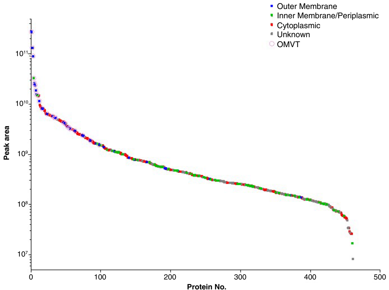
Figure 2. Relative amount of protein as determined from peak area of tandem mass spectrometry data. Proteins were assigned to a group using CELLO 27,28 and PSORTb 26 informatic tools, where the predictions differed proteins were analysed manually using UNIPROT and available published data to define a location. Where a location could not be predicted proteins were assigned an unknown status.
