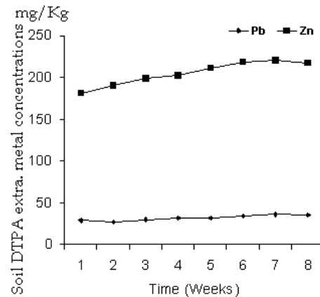
Fig 1. Variation of DTPA extractable metal concentrations during incubation time
