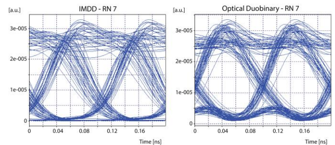
Fig. 13. Eye diagrams for RN no. 7
