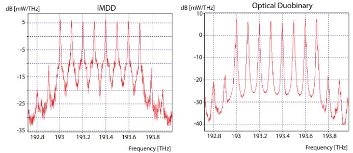
Fig. 11. Output optical spectrum for IMDD and duobinary modulation
