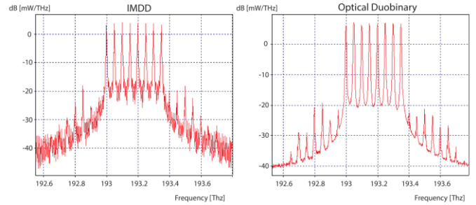
Fig. 14. Output optical spectrum for 50 GHz channel spacing
