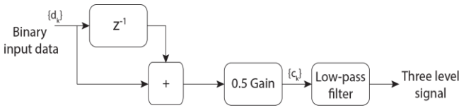
Fig. 4. Duobinary precoder
