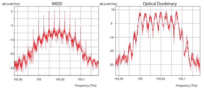
Fig. 16. Output optical spectrum for 12.5 GHz channel spacing
