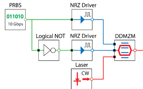
Fig. 7. Optical duobinary transmitter
