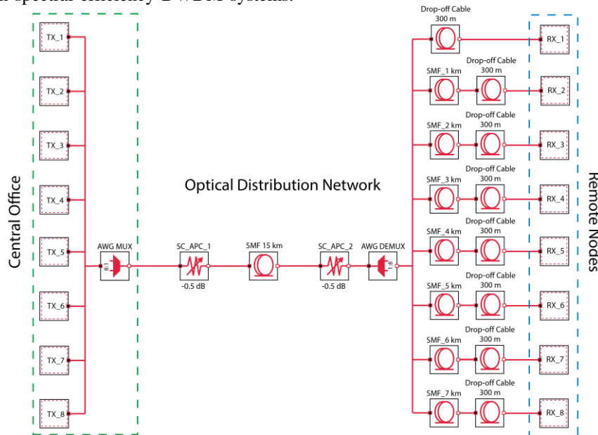
Fig. 5. Structure of proposed 10 Gbps DWDM-PON
