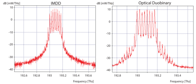
Fig. 15. Output optical spectrum for 25 GHz channel spacing
