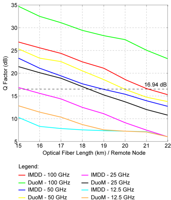
Fig. 17 Q factor vs optical fiber length for various channel spacings
