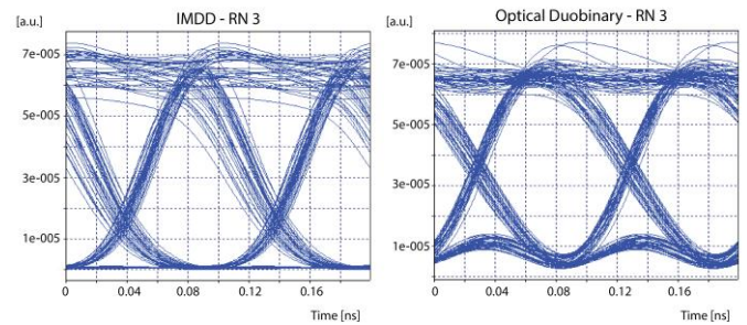
Fig. 12. Eye diagrams for RN no. 3
