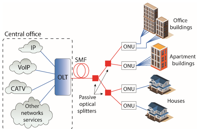
Fig. 1. Structure of passive optical network
