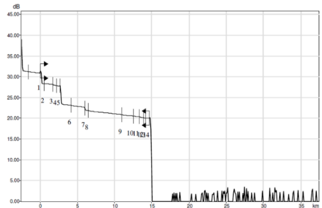
Fig. 8. The reflection curve of the real ODN
