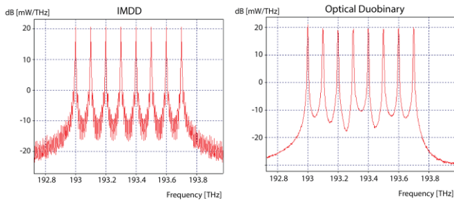
Fig. 10. Input optical spectrum for IMDD and duobinary modulation
