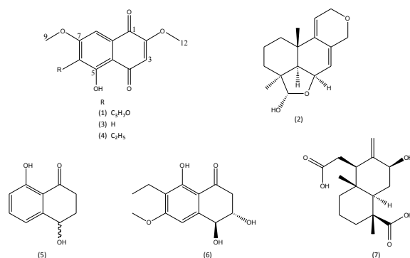
Figure 1. Isolated compounds of B. australis .
