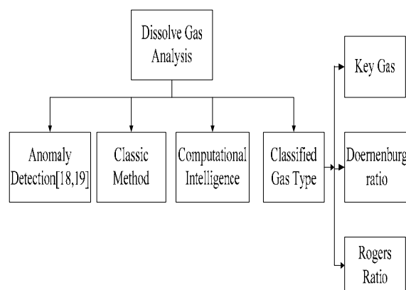
Fig. 3. Classification of dissolved gas analysis activities.
