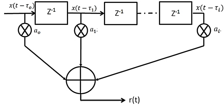
Fig. 2. Impulse response of the wireless channel.
