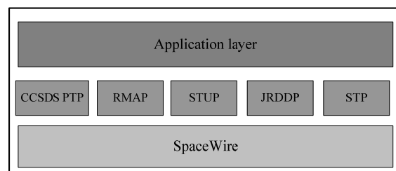
Fig. 1. Transport protocols over SpaceWire
