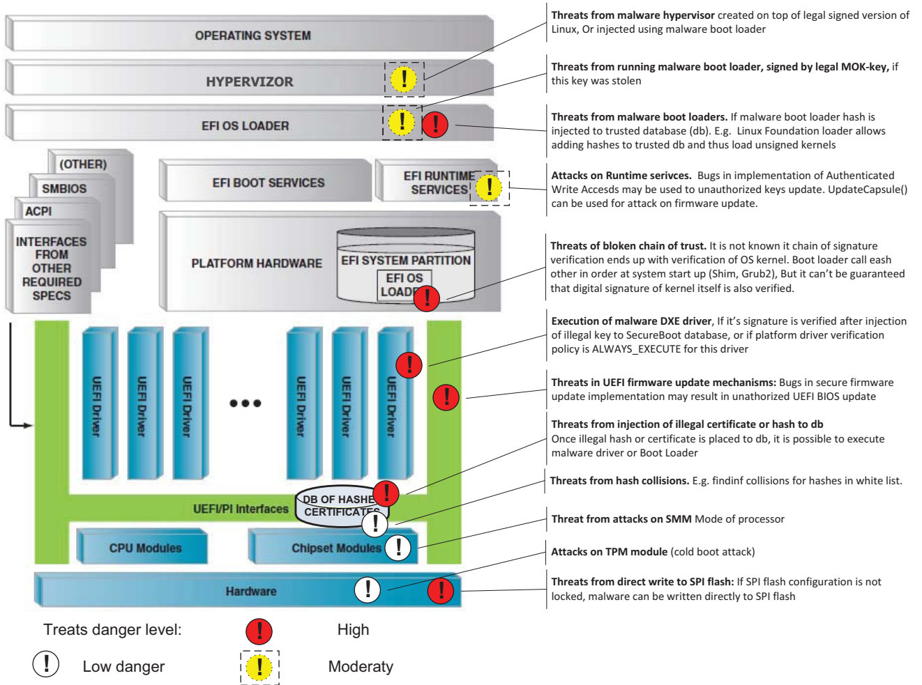
Fig. 2. UEFI threats
