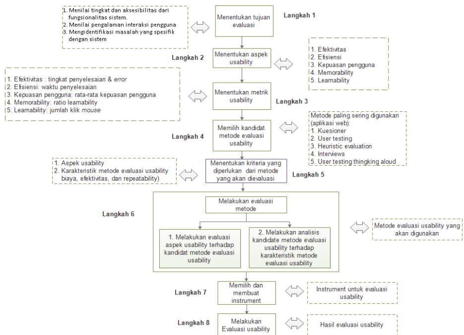
Figure 1. Proposed Framework for Usability Evaluation on E-Government
