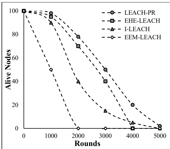
Fig.5. Comparison between I-LEACH, EHE-LEACH, EEM-LEACH, LEACH-PR presence of heterogeneity: Alive nodes vs. Rounds ( m=0.1, \alpha=1 )
