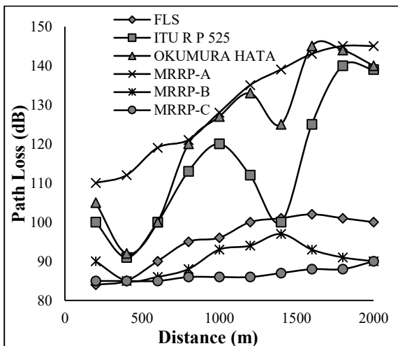
Fig.6. Path Loss predictions at 3.5GHz in Urban environment
