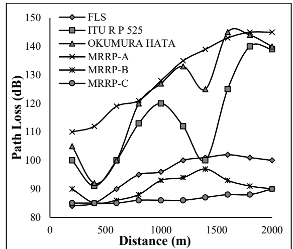
Fig.7. Path loss predictions at 3.5GHz in rural environment
