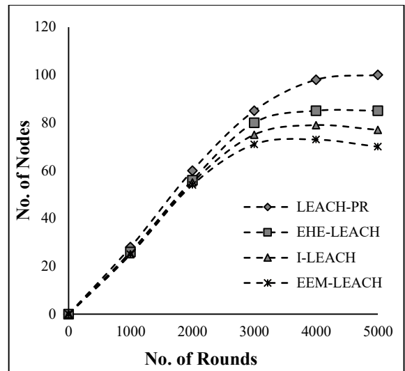
Fig.4. Comparison between I-LEACH, EHE-LEACH, EEM-LEACH, LEACH-PR presence of heterogeneity: No. of Nodes vs. Rounds (for 5000 Rounds)
