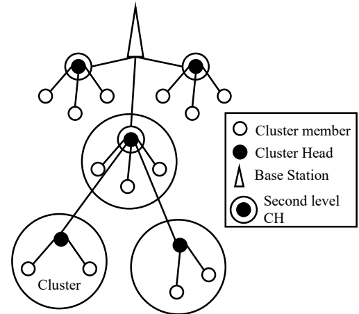
Fig.3. Clustering Topology of TEEN
