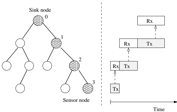
Fig. 5. An example of the proposed scheduling scheme.
