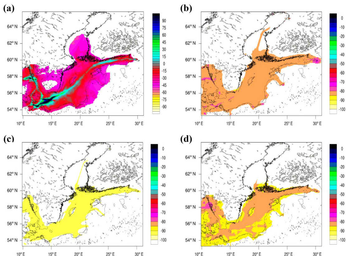
Figure 8. Future (2040) change in the ship-related contribution in summer (JJA) in percent compared to 2012, given as the relative difference between the ship contribution from the BAU 2040 simulation and the ship contribution from the present-day simulation: (a) daily maximum \text{O}_3 , (b) \text{NO}_2 , (c) \text{SO}_2 and (d) \text{PM}_{2.5} . Not coloured (empty) areas indicate grid cells with a ship contribution in BAU 2040 of less than 1.0 ppbv, 0.1 ppbv, 0.01 ppbv and 0.005 \mu\text{g m}^{-3} , for daily max \text{O}_3 , \text{NO}_2 , \text{SO}_2 and \text{PM}_{2.5} , respectively. Ship-related contribution only shown for the high-resolution area. Note the different scale for daily max \text{O}_3 (from -100\% to 100\% ).
