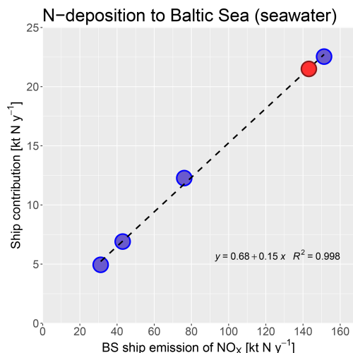
Figure 12. Relationship between emissions of \text{NO}_x (in \text{kt N yr}^{-1} ) from the Baltic Sea ship fleet and the annual ship-related nitrogen deposition (in \text{kt N yr}^{-1} ) to the Baltic seawater (on spatial average) based on the model results of the present-day simulation and the model results of the future scenario simulations. Red-filled circle indicates the ship contribution in scenario SSP3 predicted from the linear fit to the relationship.
