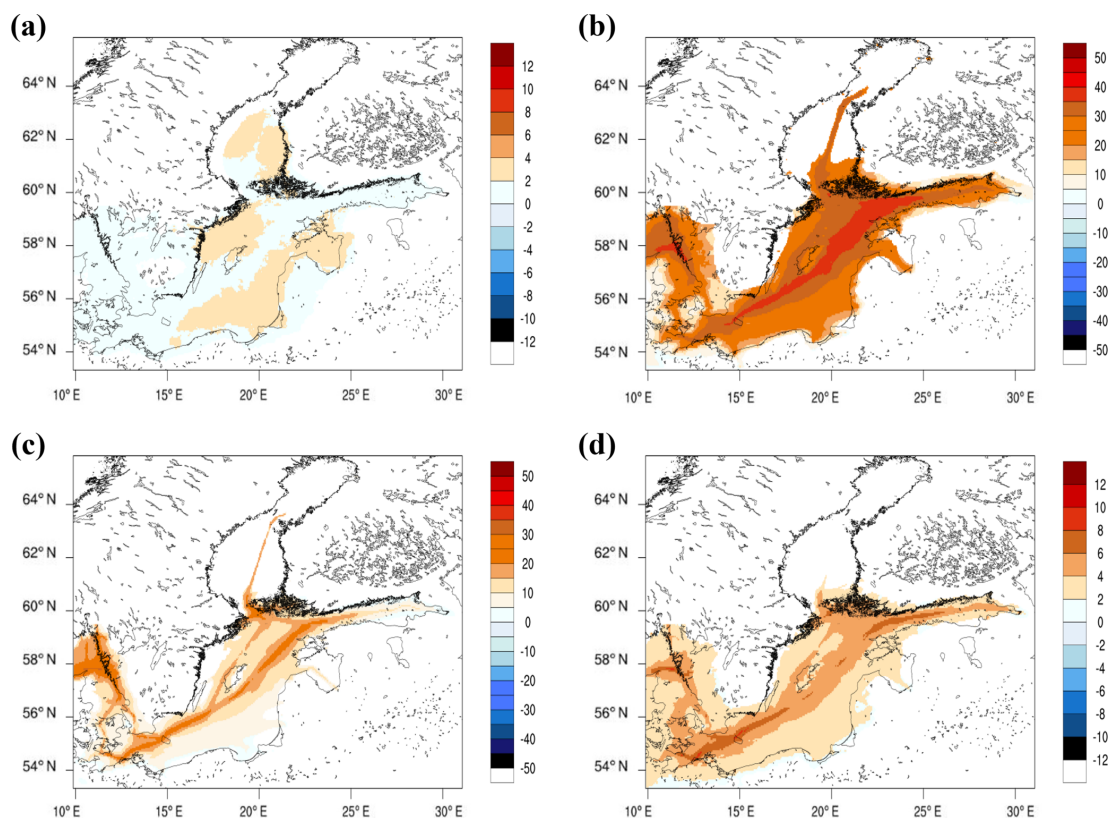
Figure 10. Effect of lower fuel efficiency on the future air quality in summer (JJA) 2040 in the Baltic Sea region as relative difference (in percent) between the scenario simulations EEDI 2040 and BAU 2040: (a) daily maximum O 3 , (b) NO 2 , (c) SO 2 and (d) PM 2.5 . Not coloured (white) areas indicate grid cells with ship contribution in BAU 2040 of less than 1.0 ppbv, 0.1 ppbv, 0.01 ppbv, 0.005 \mu\text{g m}^{-3} , for daily max O 3 , NO 2 , SO 2 and PM 2.5 , respectively.
