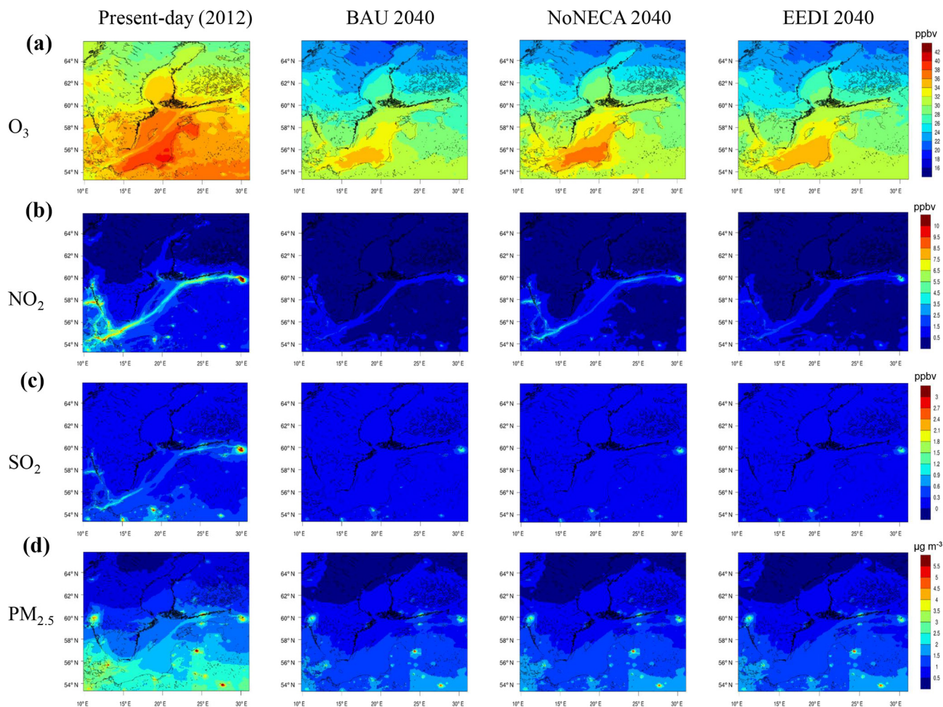
Figure 6. Future air quality situation in the Baltic Sea region in summer (JJA) compared to the present day. CMAQ model results for present-day (first column), for BAU 2040 (second column), for NoNECA 2040 (third column) and for EEDI 2040 (fourth column) are shown for (a) daily maximum O_3 , (b) NO_2 , (c) SO_2 and (d) PM_{2.5} .
