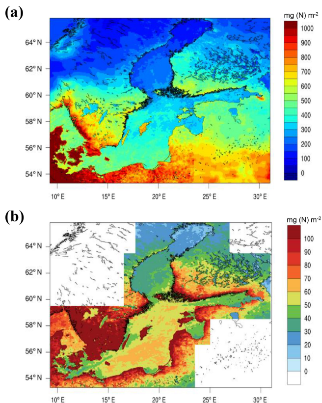
Figure 4. Present-day (2012) accumulated total deposition of nitrogen (in \text{mg(N)m}^{-2} ) in the Baltic Sea region from CMAQ model results: (a) annual deposition and (b) annual ship-related deposition. Ship contribution is only shown for the high-resolution area.
