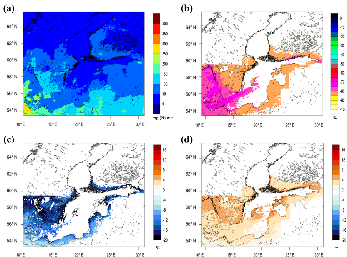
Figure 11. Nitrogen deposition in summer (JJA) 2040: (a) accumulated total deposition of nitrogen (in \text{mg}(\text{N}) \text{m}^{-2} ) in scenario BAU 2040, (b) percentage change in the ship contribution to nitrogen deposition in scenario BAU 2040 compared to the present day, (c) effect of the NECA on nitrogen deposition, and (d) effect of the lower efficiency of EEDI on nitrogen deposition. Not coloured (empty) areas indicate grid cells with ship contribution in BAU 2040 of less than 6.0 \text{ mg}(\text{N}) \text{m}^{-2} for total nitrogen deposition. The ship-related contribution is only shown for the high-resolution area.
