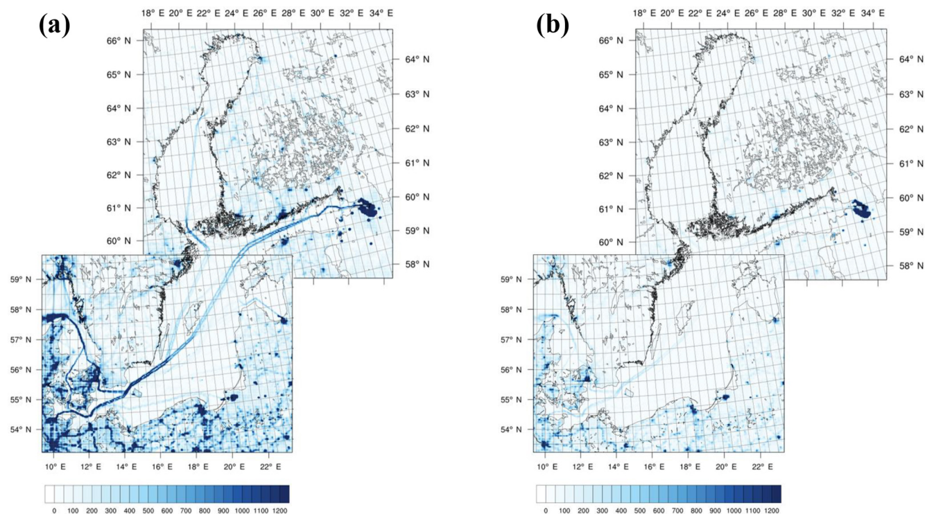
Figure 2. Annual total emissions of \text{NO}_x ( \text{mg}(\text{N}) \text{m}^{-2} ) in the surface layer for the Baltic Sea region: (a) in 2012 and (b) in 2040 for the BAU scenario. Gridded emissions from the STEAM and SMOKE emission databases interpolated to a grid resolution of 4 \times 4 \text{ km}^2 and transformed to a Lambert conformal projection for the two CMAQ high-resolution domains. Grid lines mark a lat–long grid with 0.5 \times 0.5^\circ cells.
