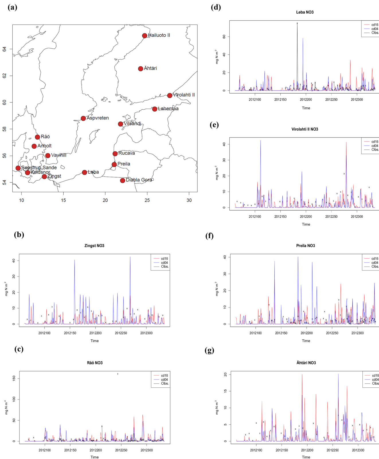
Figure 3. Comparison of modelled wet deposition of nitrate ( WNO_3 ) as daily sums (in \text{mg(N)} \text{m}^{-2} \text{day}^{-1} ) from the 16 km resolution grid (red) and 4 km resolution grid (blue) to observed daily sums (black crosses) at regional background stations around the Baltic Sea from the EMEP monitoring network: (a) map with stations as red circles, (b) Zingst, DE0009R, (c) Rää, SE0014R, (d) Leba, PL0004R, (e) Virolahti II, FI0017R, (f) Preila, LT0015R and (g) Ähtäri, FI0004R. Comparison time period: 1 March to 30 November 2012. All available data from simulations and observations are shown.
