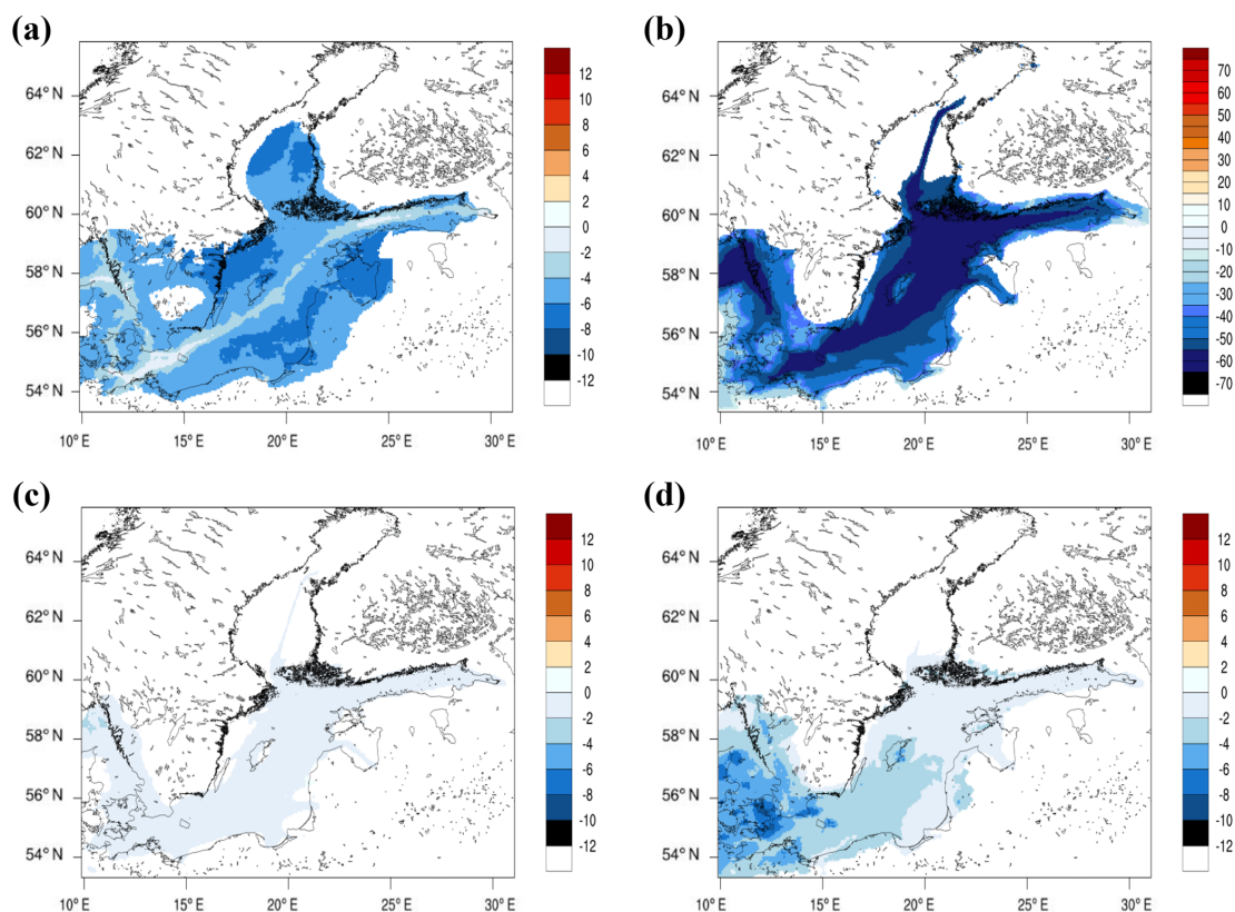
Figure 9. Effect of establishing the NECA (in 2021) on the future air quality in summer (JJA) 2040 in the Baltic Sea region as relative difference (in percent) between the scenario simulations BAU 2040 and NoNECA 2040: (a) daily maximum O 3 , (b) NO 2 , (c) SO 2 and (d) PM 2.5 . Not coloured (white) areas indicate grid cells with ship contribution in BAU 2040 of less than 1.0 ppbv, 0.1 ppbv, 0.01 ppbv and 0.005 µg m -3 , for daily max O 3 , NO 2 , SO 2 and PM 2.5 , respectively.
