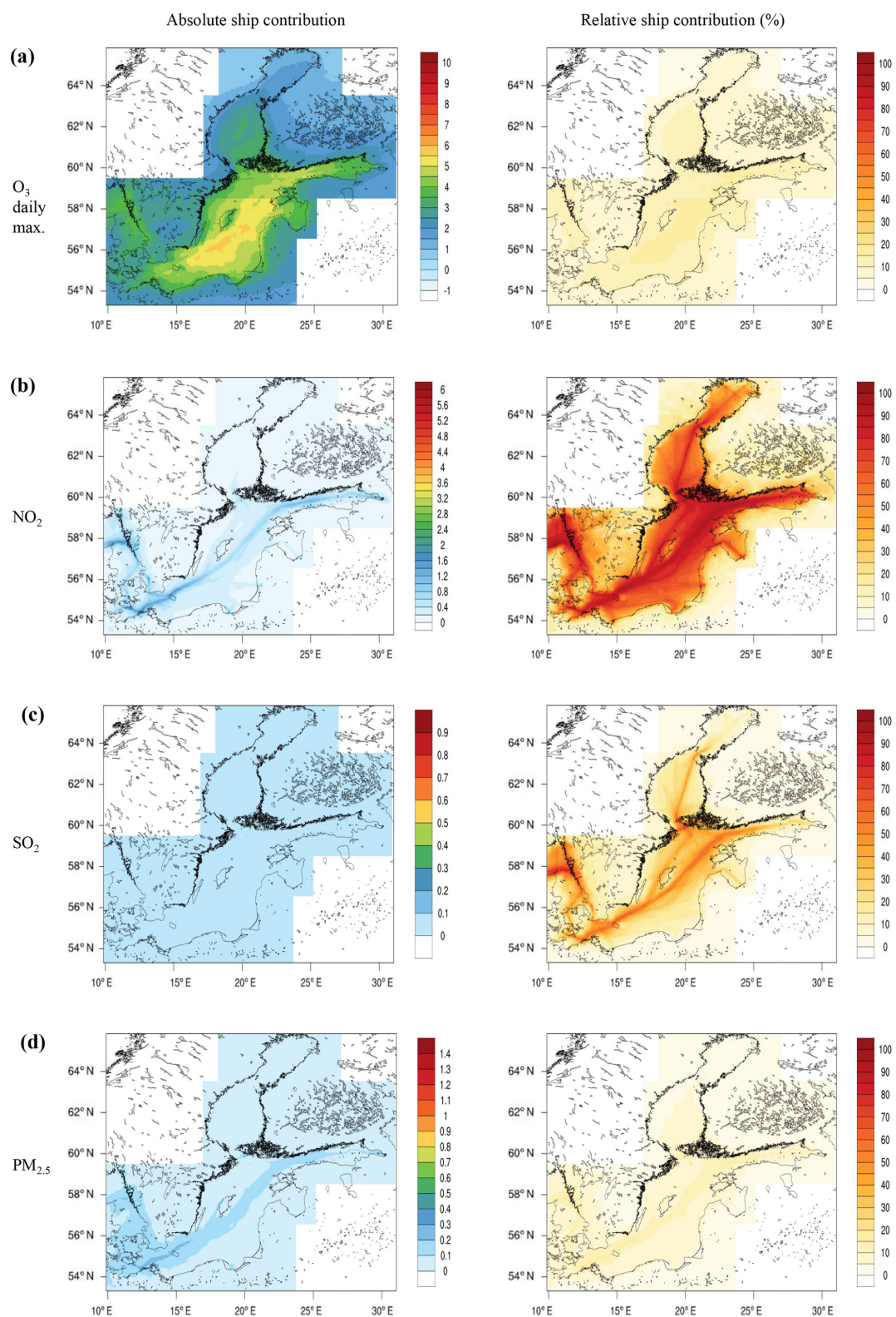
Figure 7. Future (2040) ship contribution in the Baltic Sea region in summer (JJA) from CMAQ model results for the BAU 2040 scenario: ship-related concentration (left) for gaseous pollutants (in ppbv) and for PM 2.5 (in μg m -3 ), percentage ship contribution (right) for (a) daily maximum O 3 , (b) NO 2 , (c) SO 2 , and (d) PM 2.5 . Ship-related contribution only shown for the high-resolution area. The same scales as in Fig. 5 were used to facilitate comparison of the concentration and contribution maps. The sharp change in the O 3 ship contribution north of 58.8°N is an artefact of the averaging in the overlap area of the two 4 km resolution grids.
