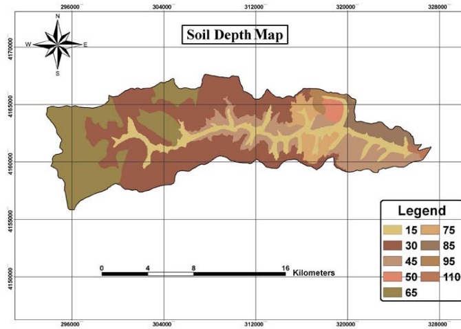
Fig 10. Soil depth of the study area (cm).
