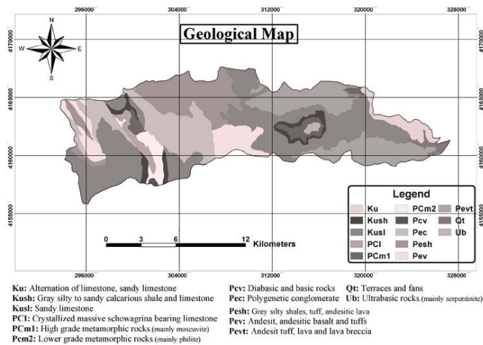
Fig 11. Geological map of the study area.
