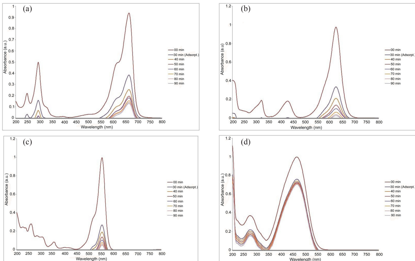
Fig. 3. UV-vis spectra for the degradation of (a) MB, (b) BG, (c) RhB, and (d) MO using the BaTiO 3 /TiO 2 -graphene nanocomposites as a photocatalyst under UV irradiation at 254 nm.
