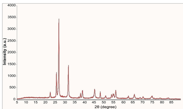
Fig. 1. XRD pattern of the BaTiO 3 /TiO 2 -graphene nanocomposites.
