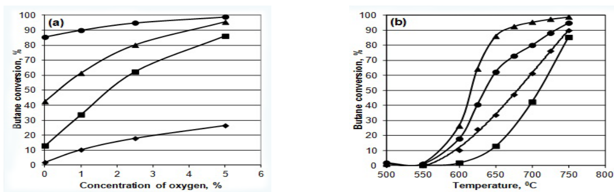
Fig. 8. Conversion of n -butane at different temperatures as a function of initial concentration of oxygen (a) ( T = 600\text{ }^{\circ}\text{C} (◆), 650\text{ }^{\circ}\text{C} (■), 700\text{ }^{\circ}\text{C} (▲) and 750\text{ }^{\circ}\text{C} (●)) and at different initial concentration of oxygen as a function of temperature (b) ( [\text{O}_2] = 0\% (■), 1\% (◆), 2.5\% (●) and 5\% (▲)) ( [\text{n-C}_4\text{H}_{10}] = 5\% , t_r = 2\text{ s} , balanced by \text{N}_2 ) [17].
