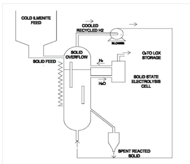
Fig. 2. Schematic representation of the process for the production of oxygen from ilmenite (adapted from [20]).
