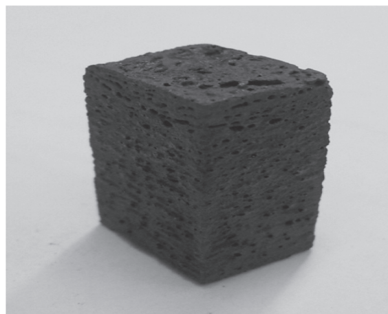
Fig. 3. Example of final parallelepiped sample obtained by the proposed patented process [72].
