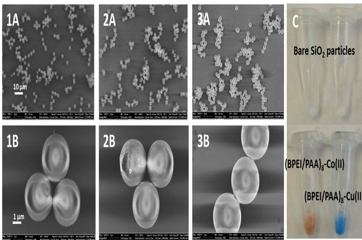
Fig. 8. SEM images (a, b) and optical images (c) of bare silica particles (with diameter 4 \pm 0.2 microns), as well as the particles with deposited (\text{BPEI/PAA})_8 and loaded \text{Co}^{2+} and \text{Cu}^{2+} ions.
