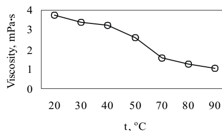
Fig. 2. The dependence of viscosity for 5 % aqueous solution of the carboxymethyl cellulose from powder cellulose on temperature.
