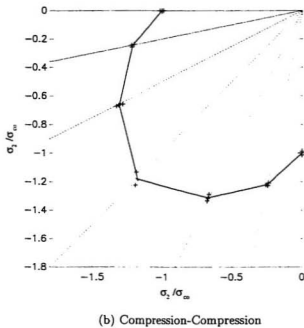
Figure 5.2: Biaxial strength envelopes for NSC under combined tension and compression, biaxial tension and biaxial compression
