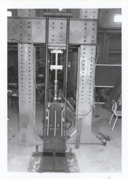
Figure 4.1: Test set-up (frontal view)
