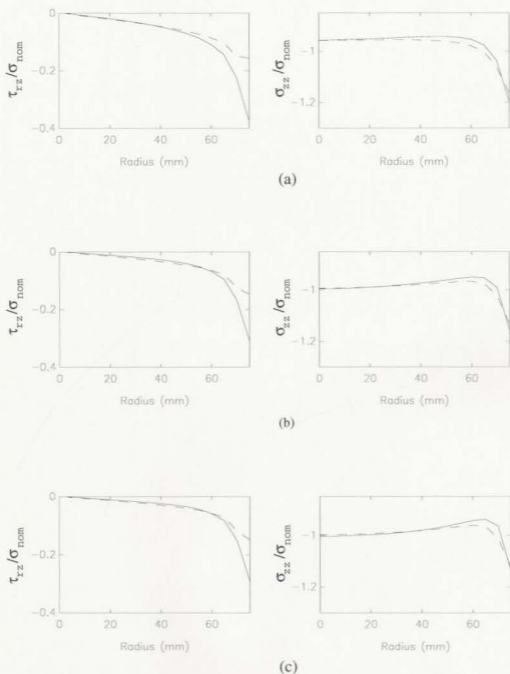
Figure 7.11: Shear stress induced in the specimen, along cylinder end, 150 \times 300 mm cylinders that are tested with 150 mm bearing block, using different modelling assumptions, (—) assuming full bond between the platen and the specimen, (---) using interface elements: (a) f'_c = 30 MPa; (b) f'_c = 70 MPa and (c) f'_c = 100 MPa
