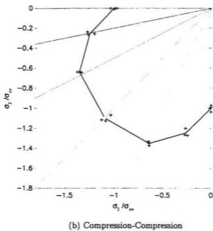
Figure 5.4: Biaxial strength envelopes for UHSC under combined tension and compression, biaxial tension and biaxial compression
