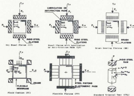
Figure 2.1: Biaxial test methods [5]
