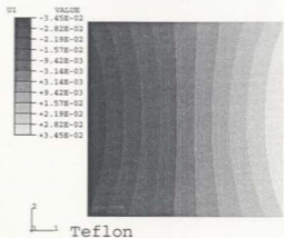
Figure 3.10: Stress contours in the direction of loading ( S22 ) and displacement contours in the orthogonal direction ( U1 ) for the uniaxial elastic analysis
