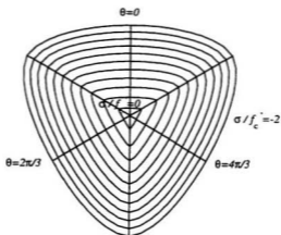
Figure 6.2: Deviatoric View of the ELM [71]
