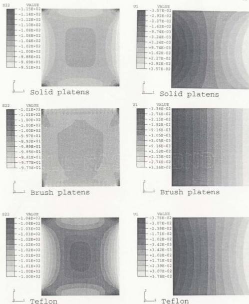
Figure 3.5: Stress contours in the direction of loading ( S_{22} ) and displacement contours in the orthogonal direction ( U_1 ) for the uniaxial cases ( f'_c = 100 MPa), at ultimate load
