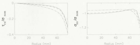
Figure 7.15: Shear stress induced in the specimen, along cylinder end, for different compressive strength, 150 \times 300 mm cylinders that are tested with 150 mm bearing block: (- · - ·) f'_c = 30 MPa; and (- - -) f'_c = 70 MPa; (—) f'_c = 100 MPa
