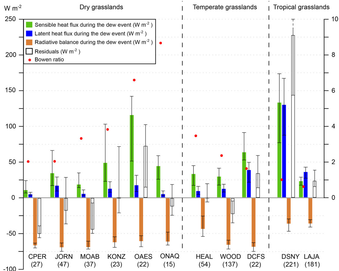
Figure 6. Median value and [25, 75] % quantiles (error bars) of the net radiation above canopy ( R_n ), and the sensible ( H ) and latent heat fluxes ( LE ) averaged during a dew event for each dewy night (indicated in parenthesis). The sign convention is positive when the grassland receives energy, and the residuals are R_n + LE + H , with R_n measured and LE and H calculated with the Monin–Obukhov similarity theory.
