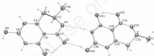
Figure 2. Asymmetric unit of the compound 1 crystals. Hydrogen bonds are indicated by dotted lines.
