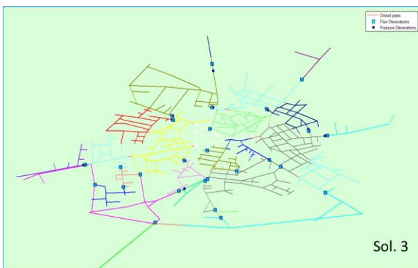
Fig. 7. DMA design solution 3.
