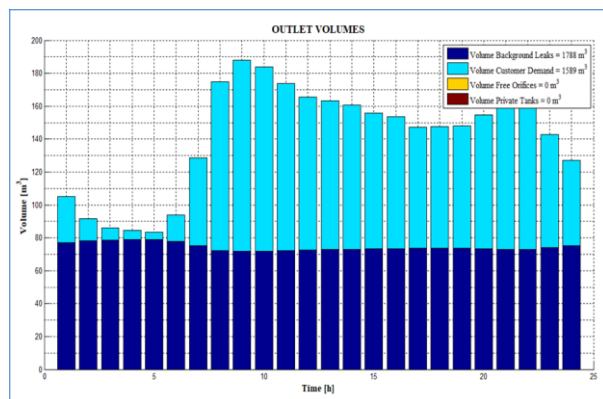
Fig. 13. Customers' demand (cyan) and volumetric real losses (blue) volumes in DMA design solution 3.
