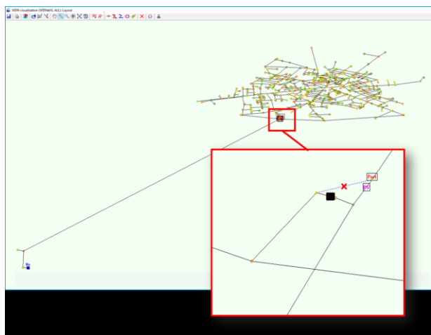
Fig. 1. WDN layout and details on feeding lines.
