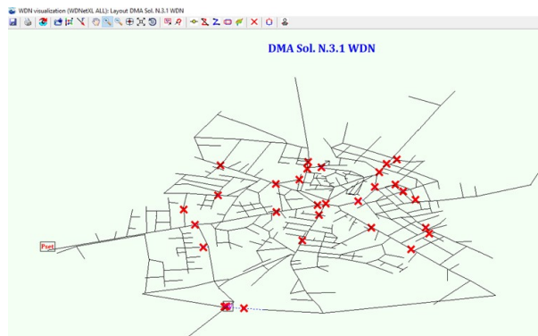
Fig. 11. Closed gate valves in DMA design solution 3.
