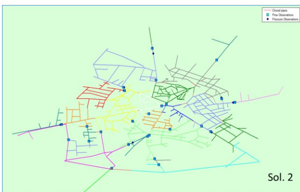
Fig. 6. DMA design solution 2.
