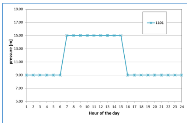
Fig. 2. Original pressure settings of the local PRV.
