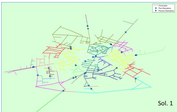
Fig. 5. DMA design solution 1.
