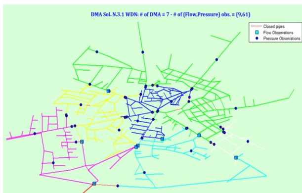
Fig. 17. Example of DMAs selected based on solution 3.
