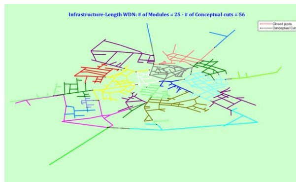
Fig. 4. Network topological segmentation .
