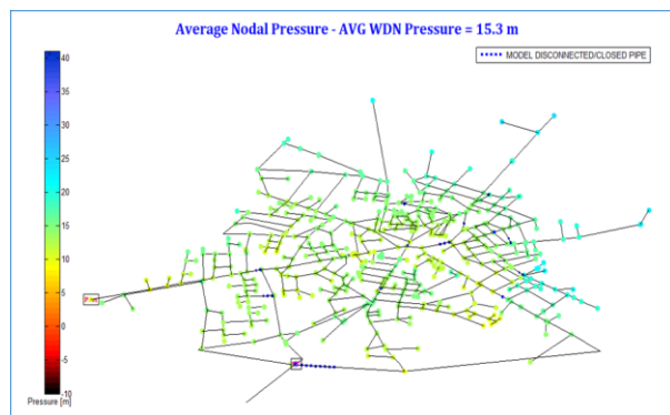
Fig. 12. Nodal pressure in DMA solution 3.
