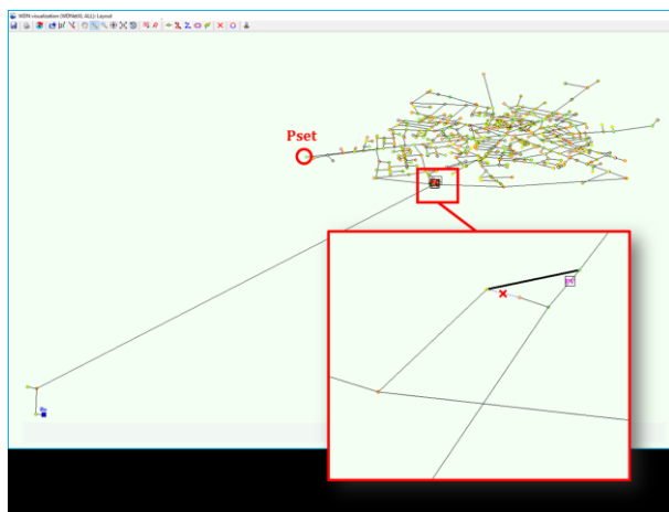
Fig. 3. New feeding configuration and location of critical node controlling RRTC PRV.
