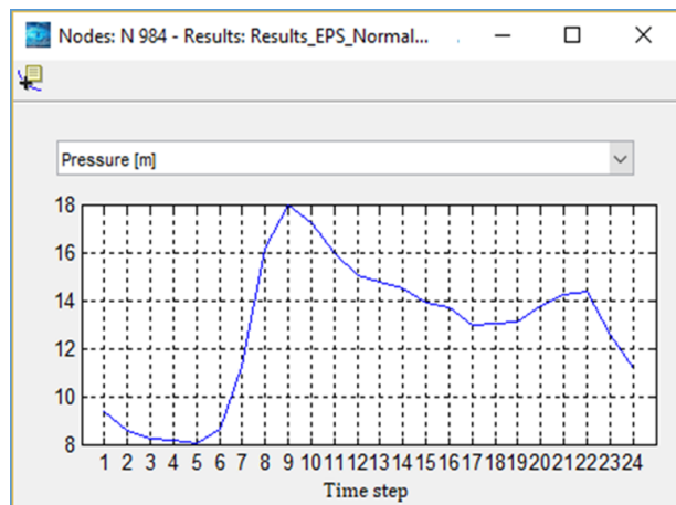
Fig. 16. Time pattern of target pressure for local PRV control node in DMA design solution 3.
