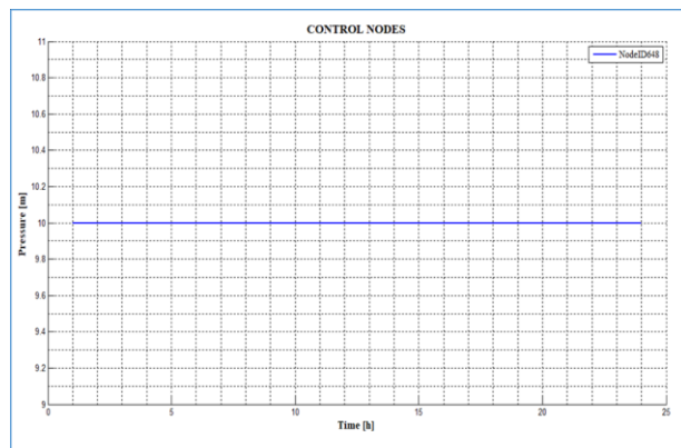
Fig. 15. Pressure at RRTC PRV control node in DMA design solution 3.
