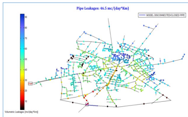
Fig. 14. Linear leakages in DMA design solution 3.
