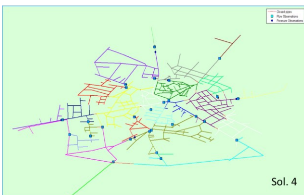
Fig. 8. DMA design solution 4.
