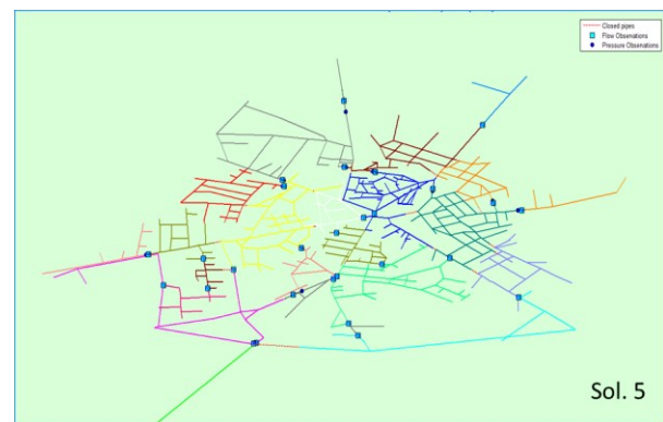
Fig. 9. DMA design solution 5.
