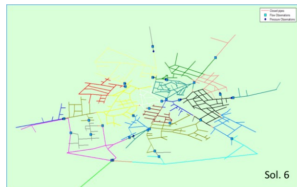
Fig. 10. DMA design solution 6.
