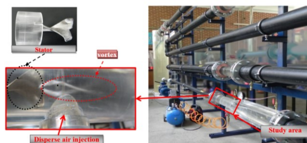
Fig. 1. Test bench for study of rotational biphasic flow with adverse pressure gradient.
