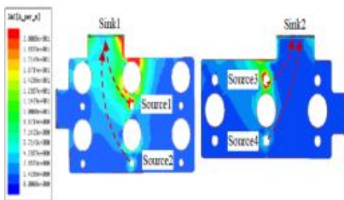
Fig. 4. Simulated current for plot model B
