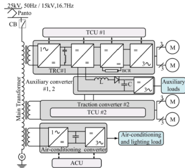
Fig. 10. EMU architecture
