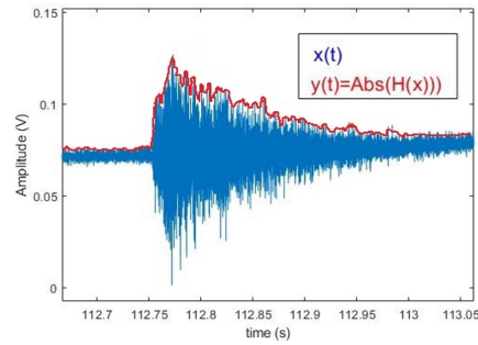
Fig. 5. Pulse signal of a typical event. In red, is represented the amplitude envelope.
