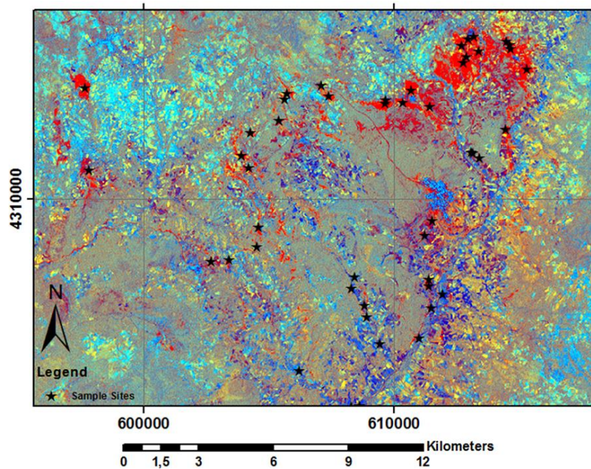
Fig.8. Sample sites shown over composite image of H and F components and PC1 from PCA of H and F components and fall in red colored areas.
