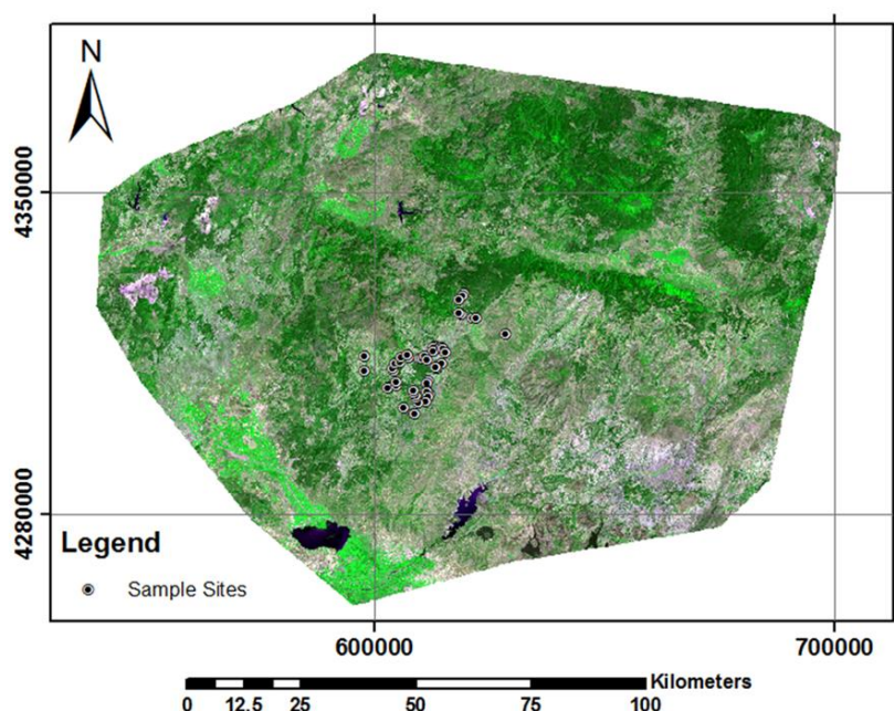
Fig. 3. LANDSAT RGB combination scene of bands respectively 2, 4 and 3 (covering sample sites).
