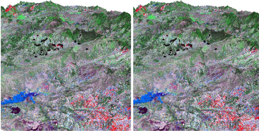
Fig. 12. Stereo visualization of sample and two other zeolite sites found after the classification.
