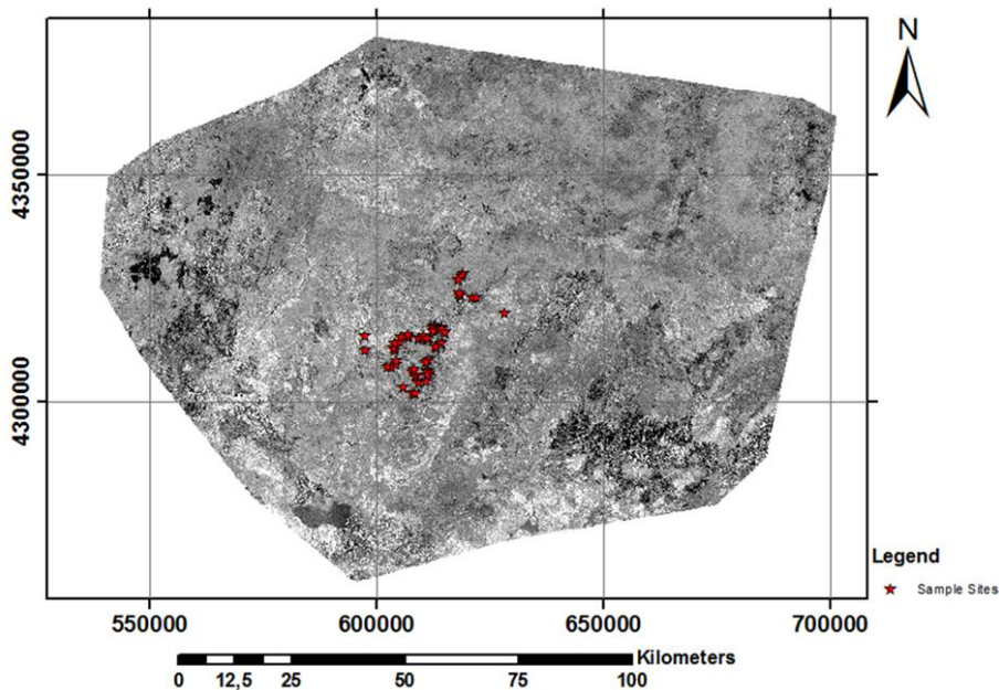
Fig. 5. Negative PC4 image of 1 st , 3 rd , 4 th and 5 th bands for Ferrite-oxide (as F component).
