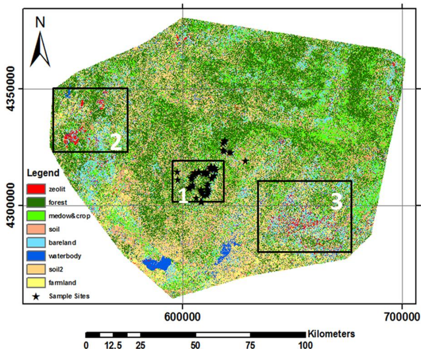
Fig. 10. General distribution of zeolites found after supervised classification over final PCA scene.
