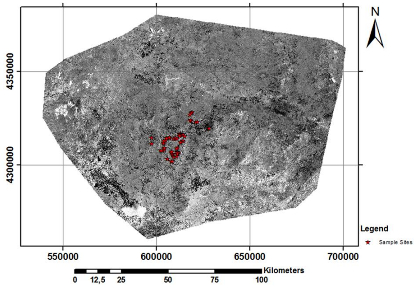
Fig. 4. Negative PC4 image of 1 st , 4 th , 5 th and 7 th bands for Hydroxide (as H component).
