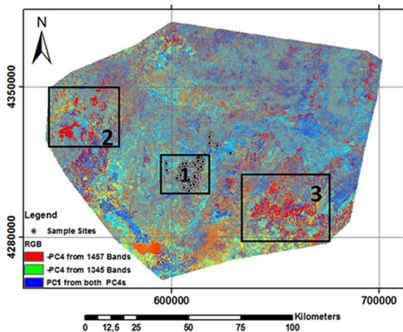
Fig. 7. Final false color composite image consisting of -PC4 from PCA of 1 st , 4 th , 5 th and 7 th bands (R), -PC4 from PCA of 1 st , 3 rd , 4 th and 5 th bands (G) and PC1 from PCA of both PC4 images (B).
