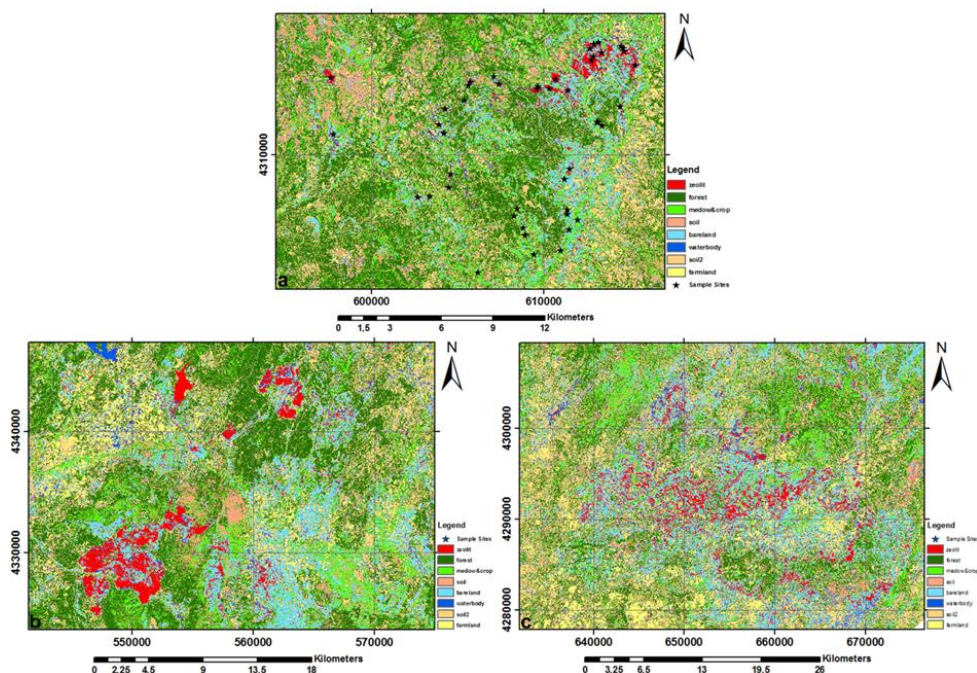
Fig. 11. Classification results of sample, 2 nd and 3 rd zeolite sites in detail.
