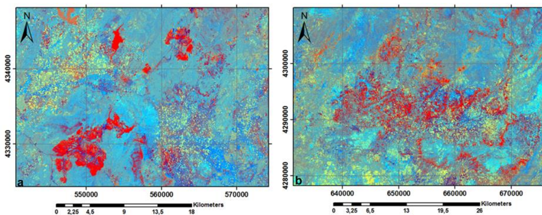
Fig. 9. Found zeolite sites and numbered as 2 nd (a) and 3 rd (b) in Fig. 7.
