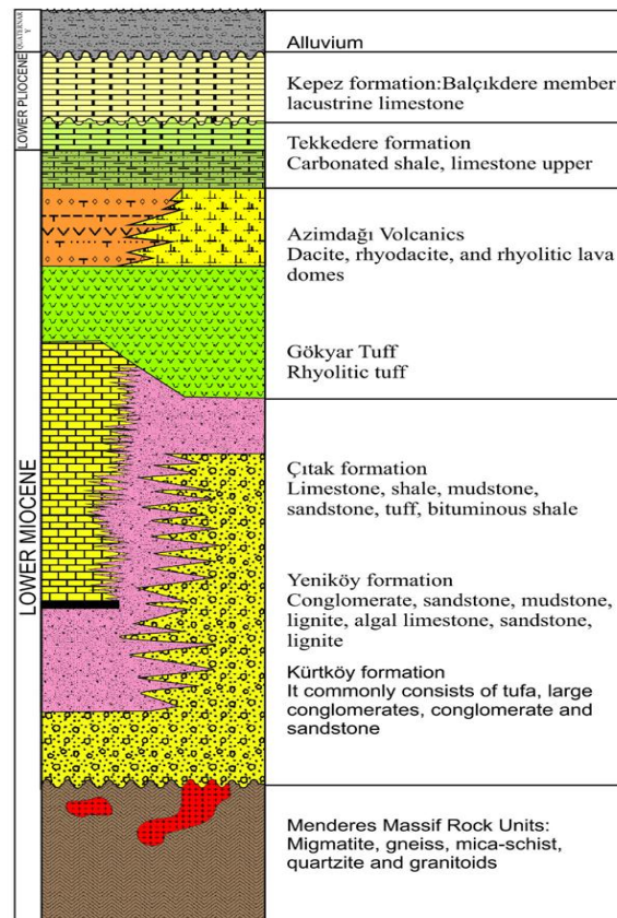
Fig. 2. Geological colon profile of Gördes and its close vicinity (taken from Göktaş 1996).
