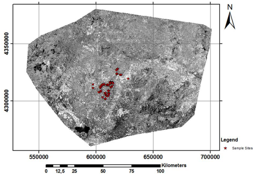
Fig. 6. PC1 from PCA of both PC4 images (H and F components).
