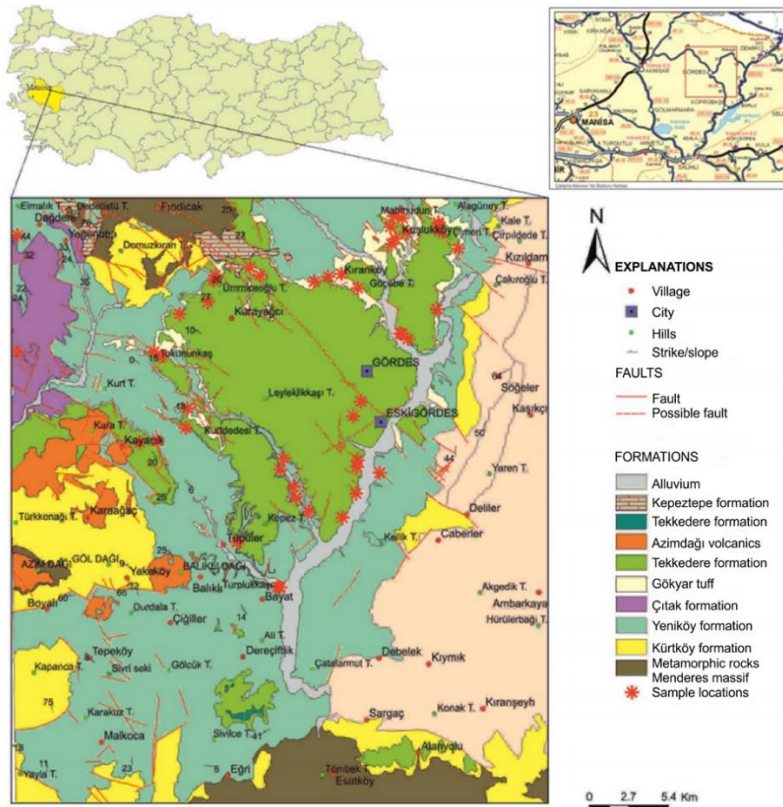
Fig. 1. Geology of the study area.
