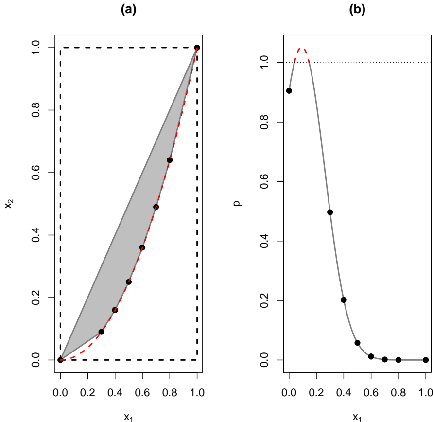
Figure 3: Examples of the (a) covariate space considered by the Fisher scoring and adaptive barrier methods (grey) compared to that considered by the EM approaches (black, dashed) for a model with a quadratic term, and (b) a hypothetical curve that produces invalid fitted risks. Observed covariate values are marked as black circles.
