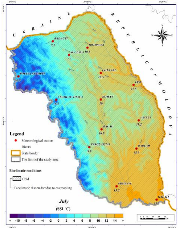
Figure 7. The spatial distribution of the SSI index in Moldova for July (1961-2013)
