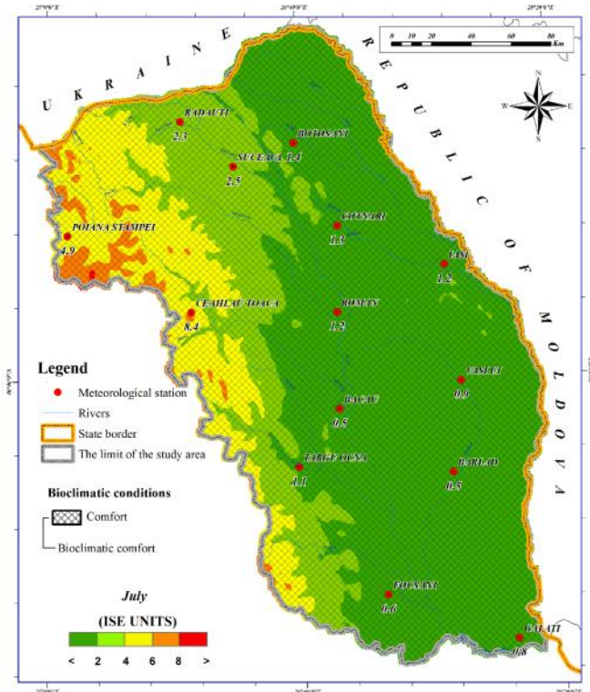
Figure 8. The spatial distribution of the ISE index in Moldova for July (1961-2013)
