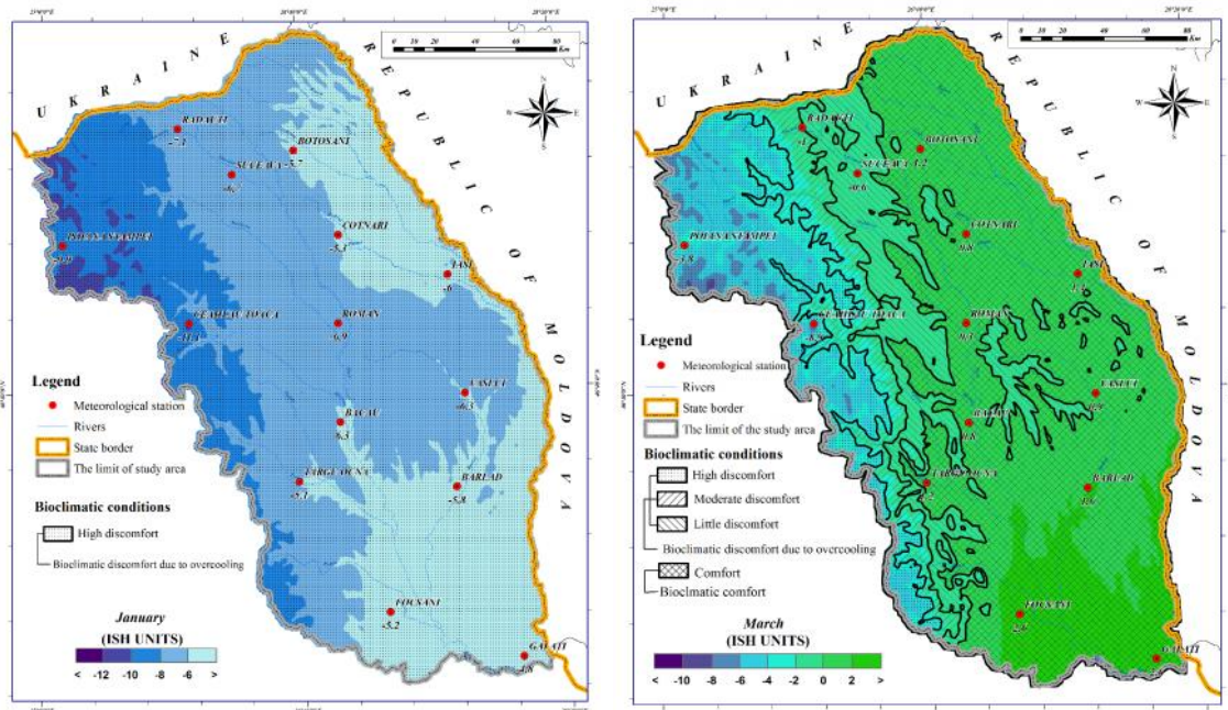
Figures 8 - 11. The spatial distribution of the ISH index in Moldova for September - Fig. 8 , November - Fig. 9 , January - Fig. 10 and March - Fig. 11 for the time interval 1961-2013
