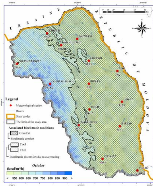
Figures 13 to 16. The spatial distribution of the Pr index in Moldova for January - Fig. 13 , April - Fig. 14 , July - Fig. 15 and October - Fig. 16 for the time interval 1961-2013.
