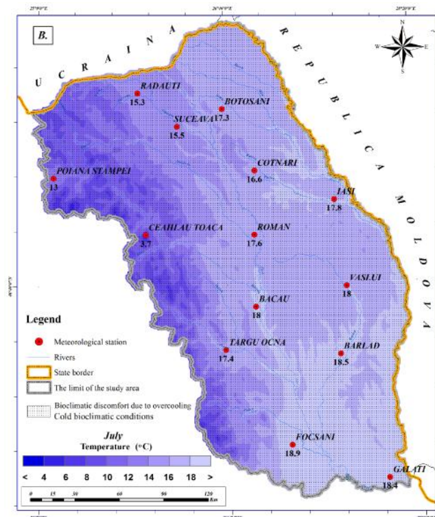
Figure 2. The spatial distribution of TEE index values in Moldova for July (1961-2013)
