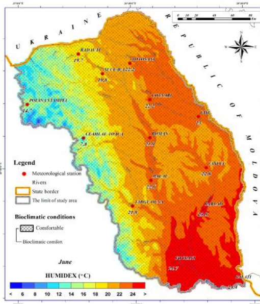
Figures 4 and 5. The spatial distribution of the HUMIDEX index in Moldova for June and July (1961-2013)
