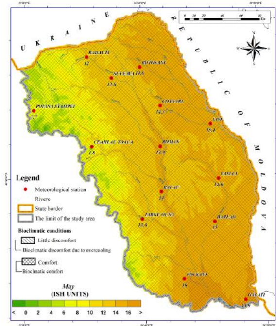
Figure 12. The spatial distribution of the ISH index for May in Moldova (1961-2013)
