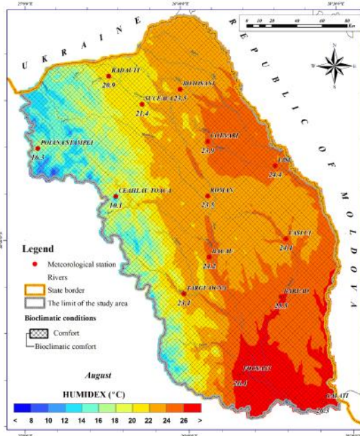
Figure 6. The spatial distribution of the HUMIDEX index in Moldova for August (1961-2013)
