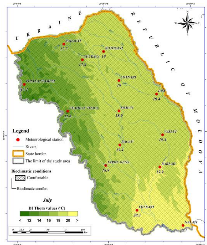
Figure. 3 The spatial distribution of DI THOM index values in Moldova for July (1961-2013) pressure of water vapor (hPa) with the formula [4].
