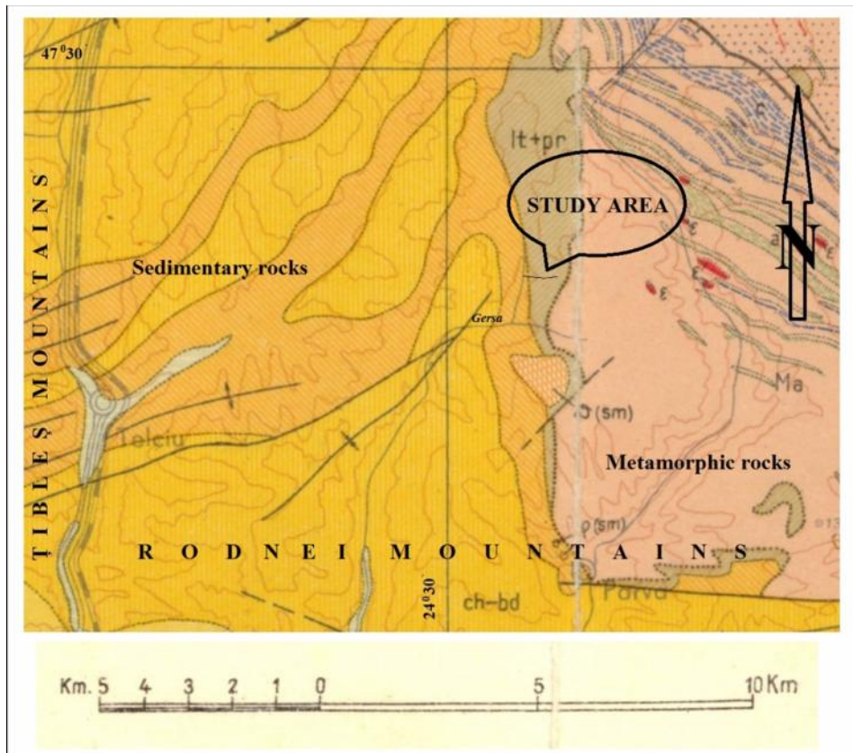
Figure 3 -Geologic map of upper Gersa River catchment area (source: Geologic Map of Romania, Vişeu file, 1:200 000 scale, 1968-with changes)
