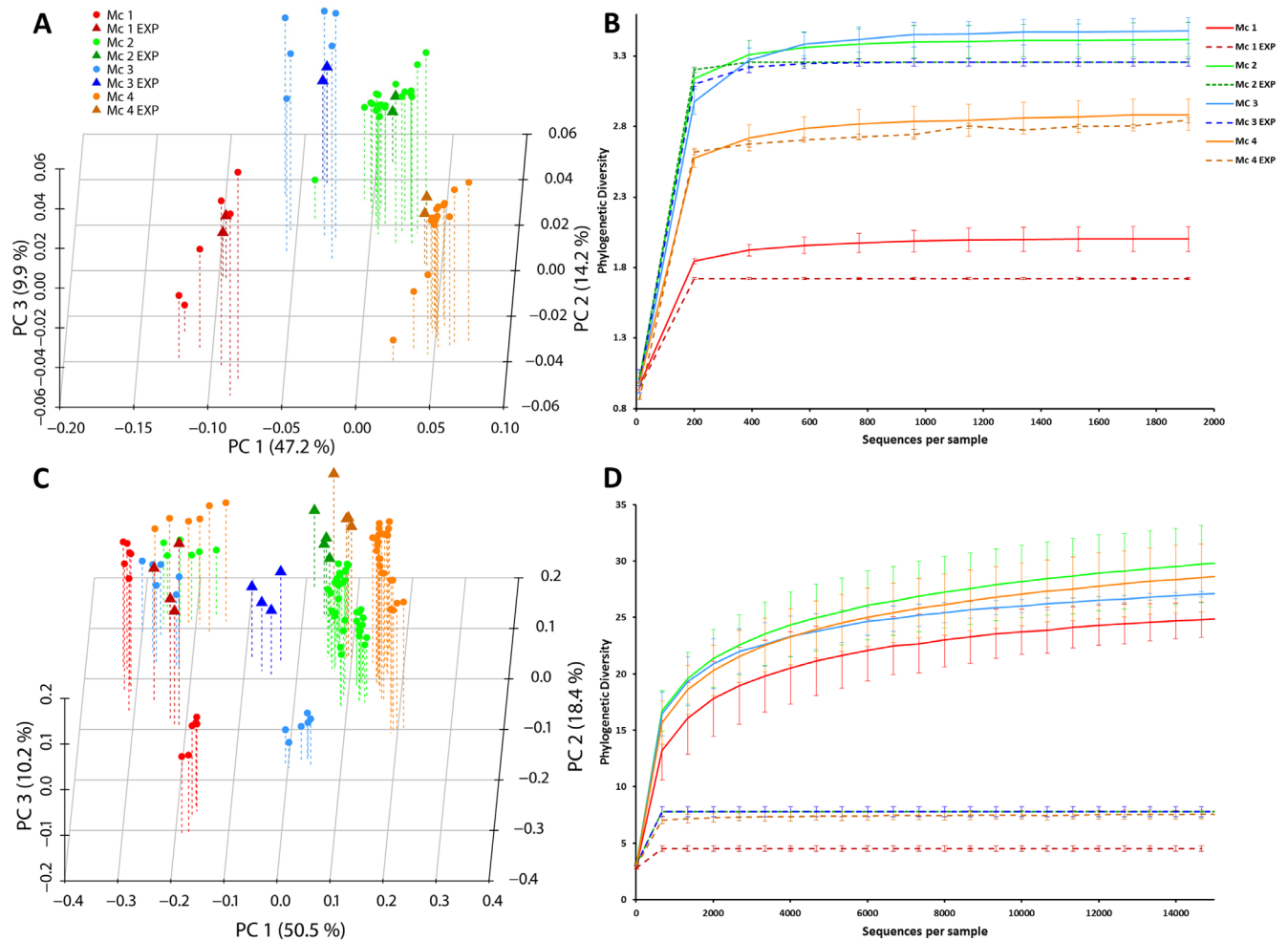
Figure 6. PCoA using Weighted Unifrac of all sequenced and expected MCs as obtained after processing of data using NG-Tax ( A ) and QIIME ( C ). Darker colored triangles represent the expected composition while lighter colored circles represent sequenced samples. B/D . Rarefaction curves of PD for all MCs and their expected counterparts for NG-Tax ( B ) and QIIME ( D ). Dashed lines represent the expected composition while solid lines represent sequenced samples.
