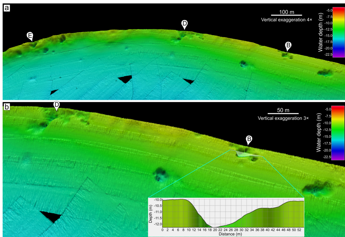
Figure 5. Multibeam bathymetric images of pockmarks. (a) Multibeam image over pockmarks E, D, and B. (b) Close-up multibeam image over pockmarks D and B. Inset shows a depth profile over pockmark B.
