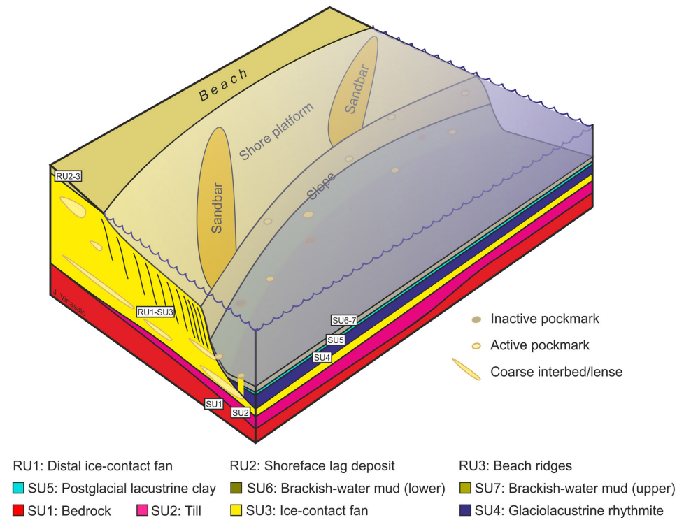
Figure 8. Summary diagrams. (a) Allostratigraphical correlation of unconformities between the onshore ground-penetrating radar and refraction seismic profiles, and the offshore seismic profiles. (b) Stratigraphical architecture of the studied submarine groundwater discharge site; not to scale.
