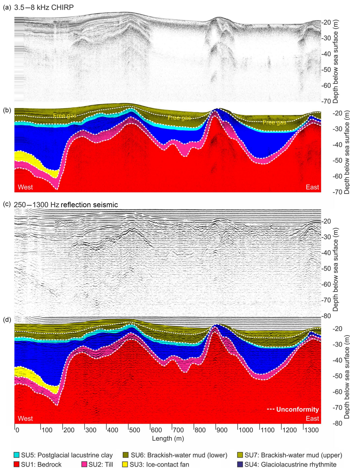
Figure 3. Offshore sub-bottom profiles collected along the survey line indicated in Fig. 1a. (a) 3.5–8 kHz CHIRP sub-bottom profile, and (b) interpretation of the profile. (c) 250–1300 Hz reflection seismic sub-bottom profile, and (d) interpretation of the profile. See text for details about the interpretation of seismic units.
