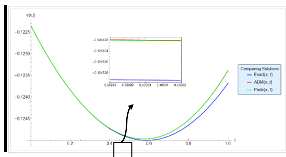
Figure 8. The curves of v(x, t) .
