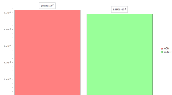
Figure 10. Bar chart of v(x, t)
