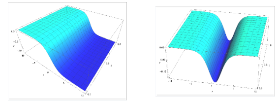
(a) u(x, t) (b) v(x, t)
