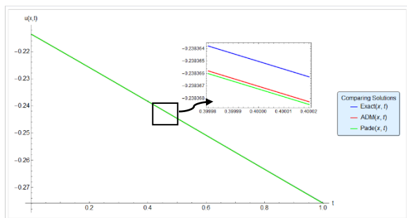
Figure 7. The curves of u(x, t) .
