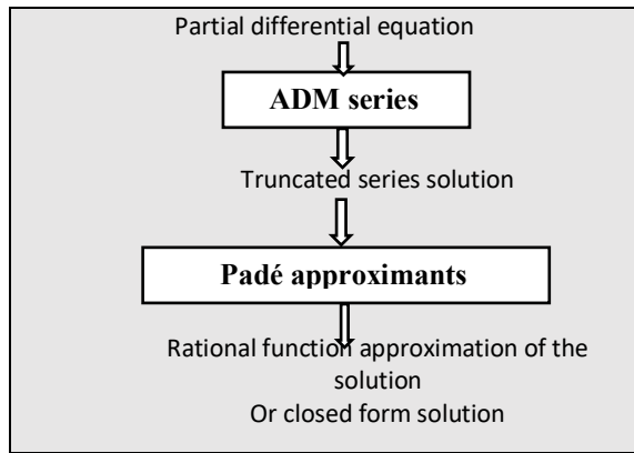
Figure 1. Flowchart of the ADM-Padé technique.
