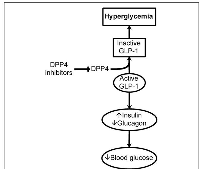
FIGURE 2 | Importance of DPP4 in hyperglycemia. Dipeptidyl peptidase IV (DPP4), or CD26, is a cell surface and soluble peptidase that can cleave the first two N-terminal amino acids from specific proteins and peptides. DPP4 is up-regulated in immune and endothelial cells as a result of inflammation seen in critically ill patients. Of specific importance to hyperglycemia, DPP4 cleaves the N-terminus of glucagon-like peptide 1 (GLP-1). GLP-1 is important in the storage and regulation of blood glucose by promoting insulin and limiting glucagon release. This cleavage of GLP-1 causes the inactivation of GLP-1 contributing to hyperglycemia. Inhibitors of DPP4 could be important in glucose control in critically ill patients with hyperglycemia.
