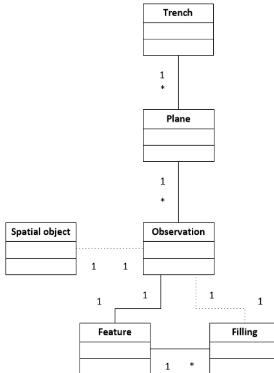
Figure 4. The observation layer, which describes the observation method for a Feature contour, and allows for linking a Feature with multiple Planes (horizontal and vertical).
