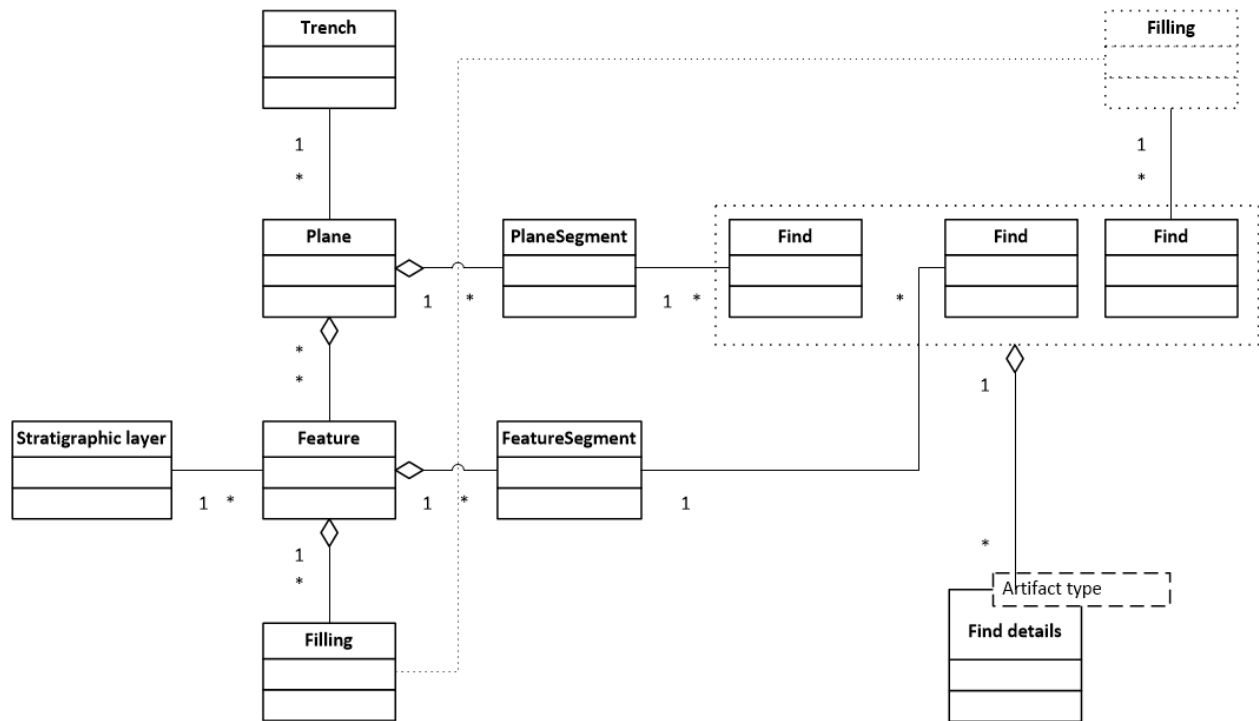
Figure 2. Basic logical data structure of the administrative objects, field observations and artifact details in a Dutch plane/feature based excavation. Note that the three Find objects represent Finds collected in a different way, but they are basically all Find objects, with the only exception that the relationship differs.
