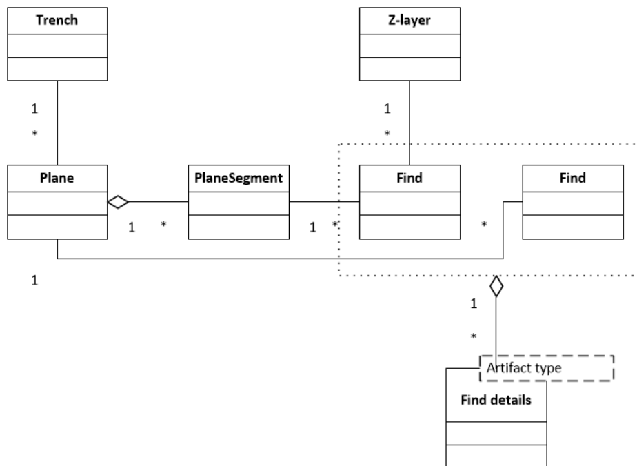
Figure 3. Logical data objects matching the field observations in a grid-wise filtering excavation.
