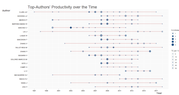
Fig. 9. Top-Authors' productivity over the time
